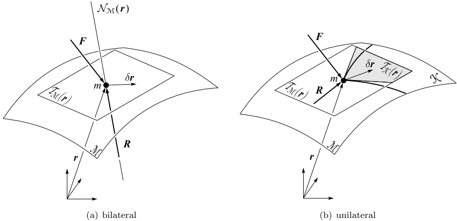
Fig. 4 Constrained point-mass
