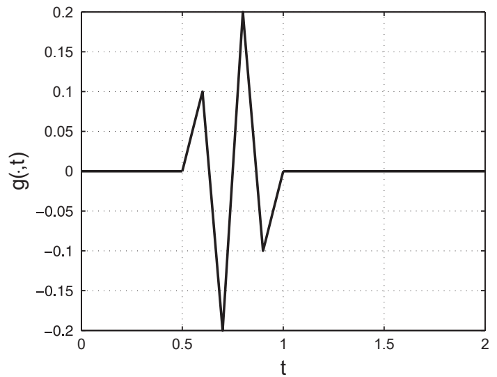
Figure 12. Dirichlet boundary condition.
