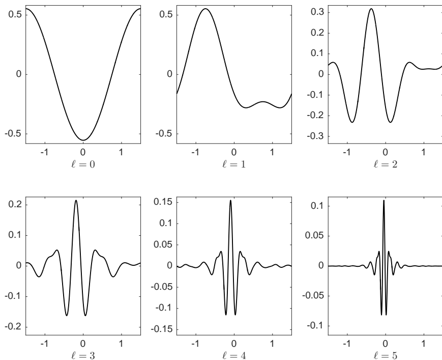
Figure 2: Wavelets \Psi_{\ell,0}^p obtained with \lambda = 1 , \nu = \frac{1}{2} , and \gamma = \frac{3}{2} , for \ell = 0, \dots, 5 .
