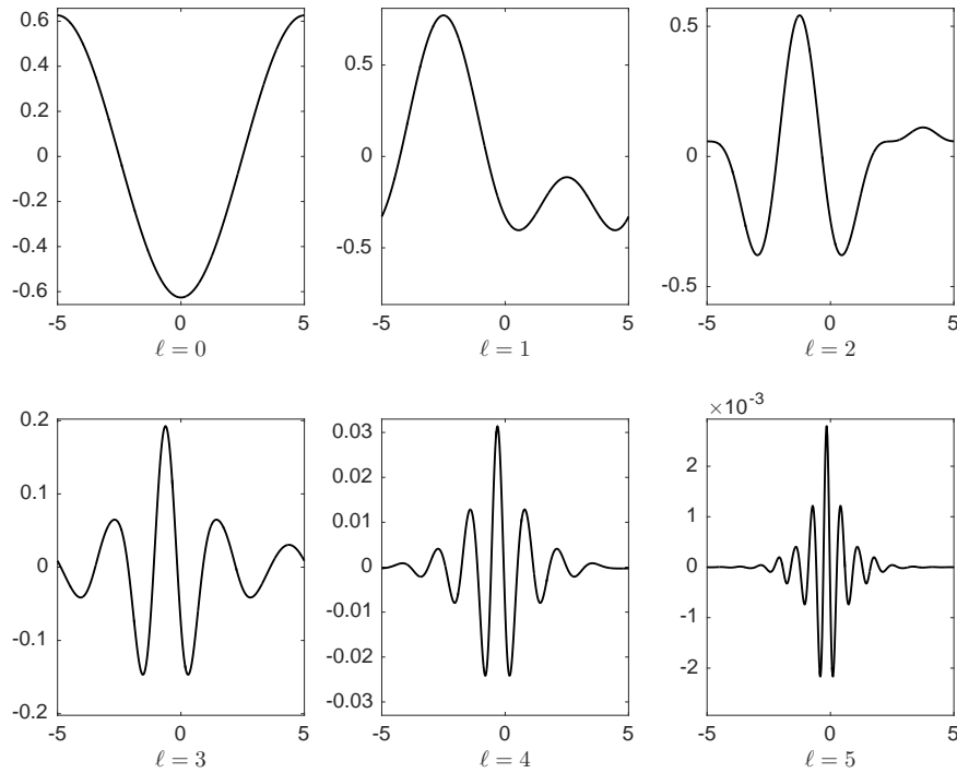
Figure 3: Wavelets \Psi_{\ell,0}^p obtained with \lambda = 1 , \nu = 4 , and \gamma = 5 , for \ell = 0, \dots, 5 .
