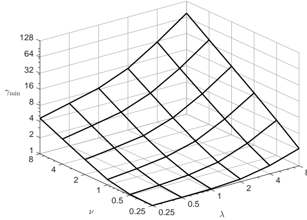
Figure 1: Numerically observed minimum value of \gamma required for positivity of \hat{k}_t , with k as in (17), in dependence on the Matérn parameters \lambda, \nu .
