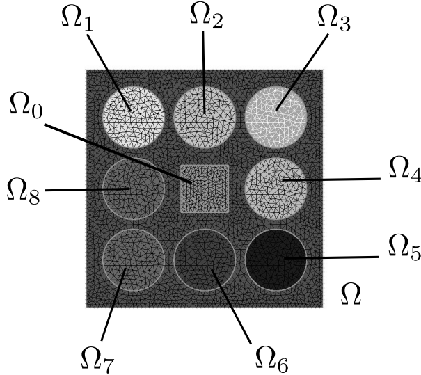
FIGURE 2. Mesh discretization and geometries of the inclusions. The domain D is the unitary square. The inner square is named D_0 , the eight circular inclusions are D_1, \dots, D_8 .
