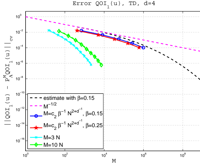
FIGURE 4. Error \mathbb{E}(\|u - \tilde{P}_m^n u\|^2) in the case d = 4 . Different relations between the number of samples n and the dimension of the polynomial space m are tested. The black dash line is the bound (119). The magenta dash line is the Monte Carlo convergence rate n^{-1/2} .
