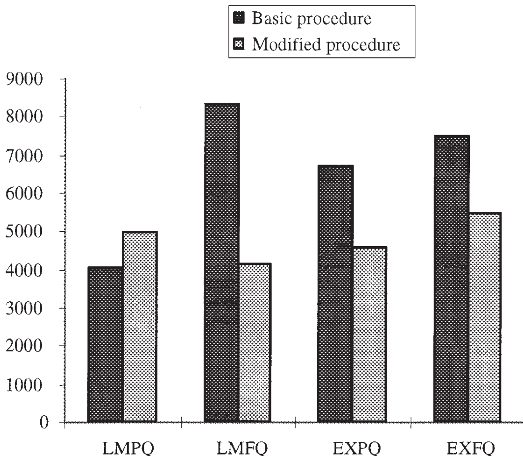
Figure 7. Times in 10^{-2} \times seconds, n = 10000 , without Problems 15.
