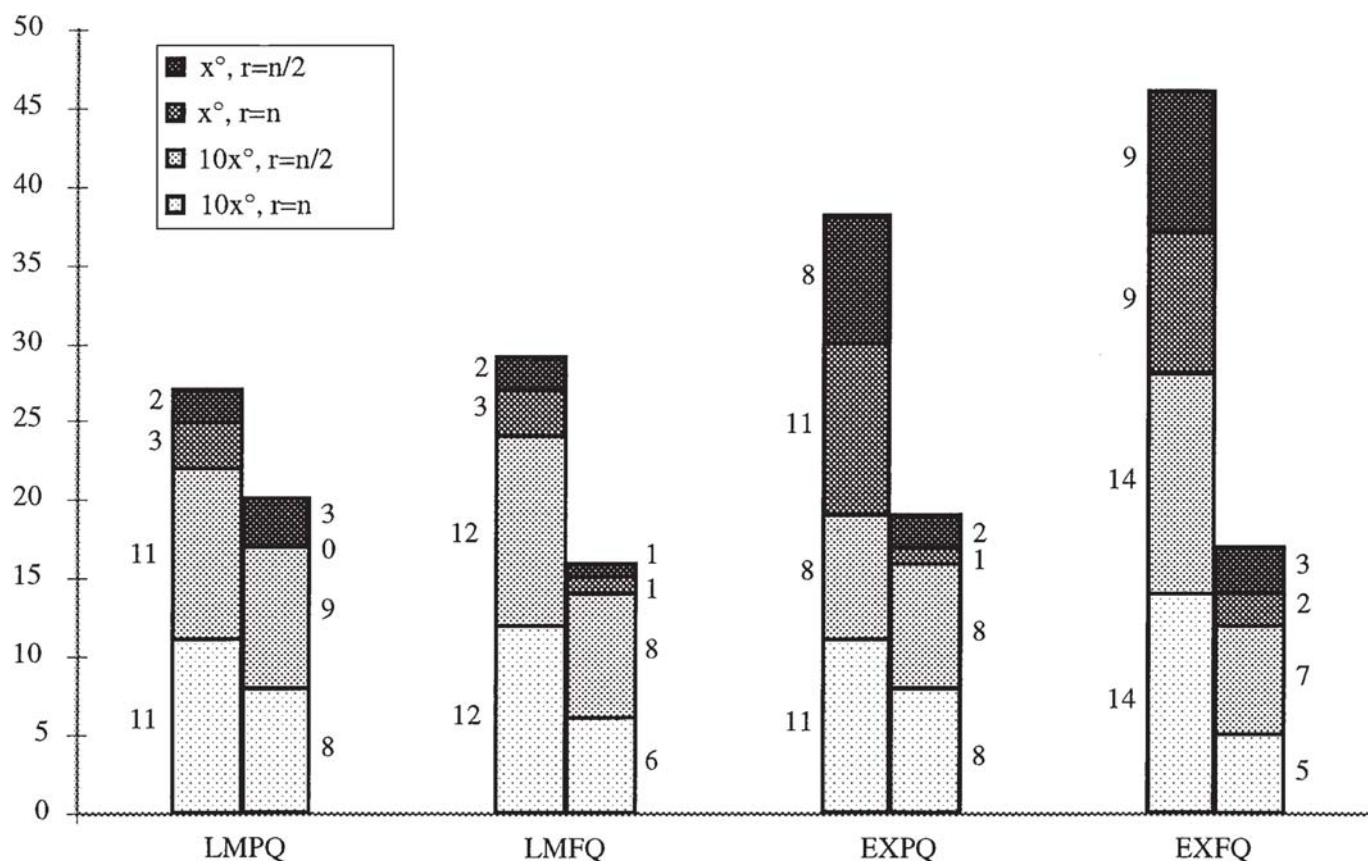
Figure 2. Failures in detail.
