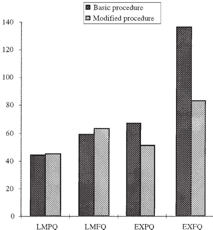
Figure 3. Times in 10^{-2} \times seconds, n = 100 .
