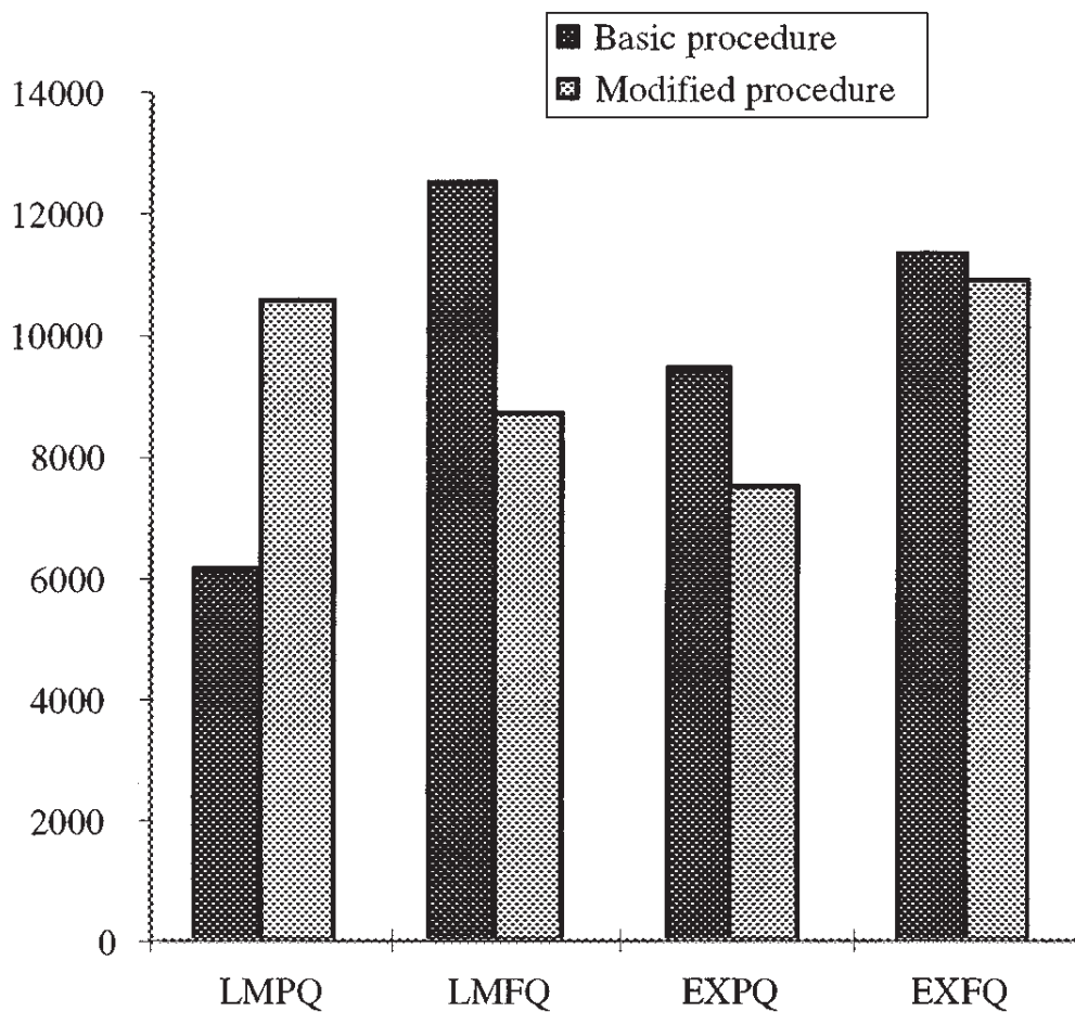
Figure 5. Times in 10^{-2} \times seconds, n = 10000 .
