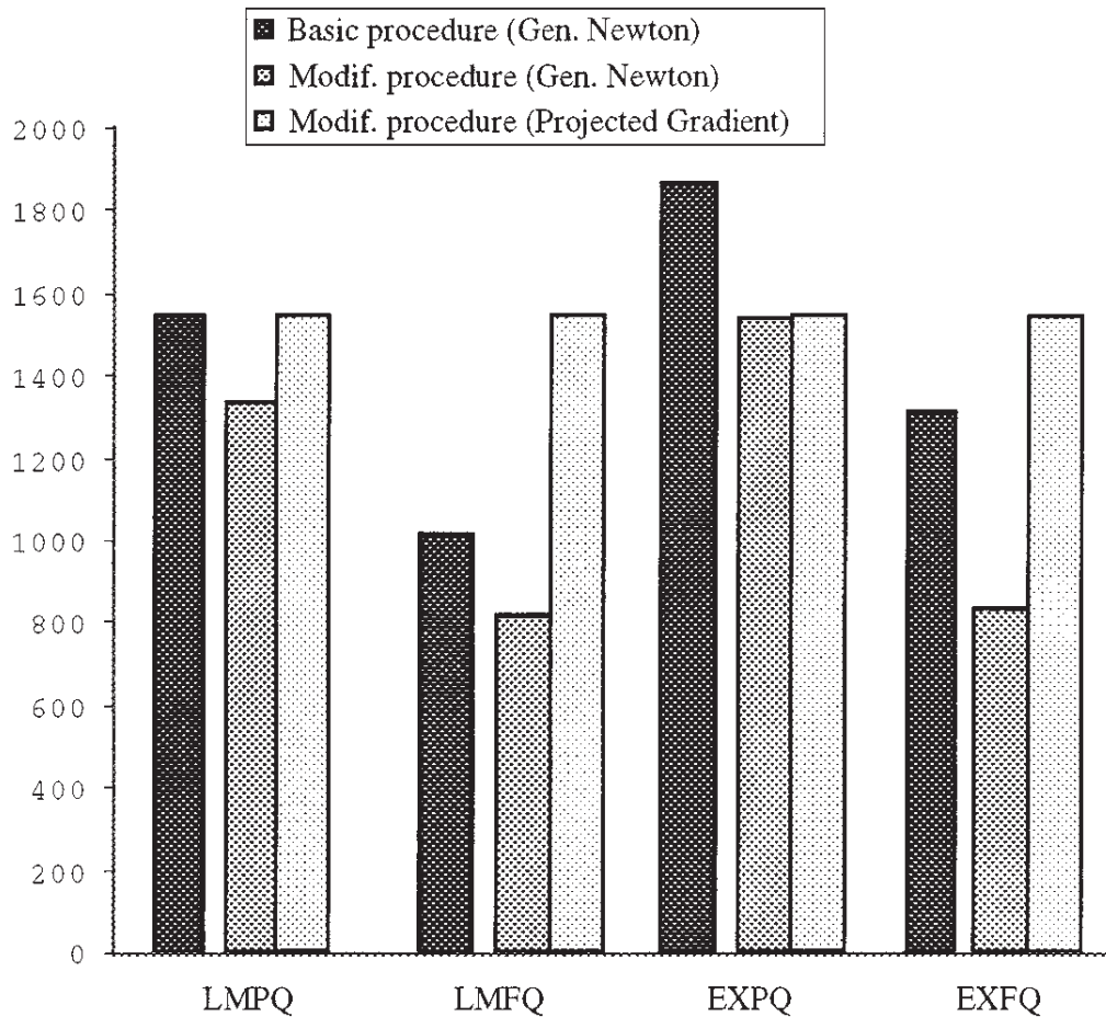
Figure 9. Number of function evaluations.
