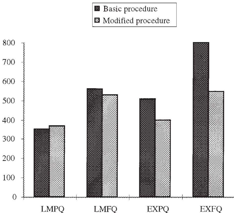
Figure 6. Times in 10^{-2} \times seconds, n = 1000 , without Problems 15.
