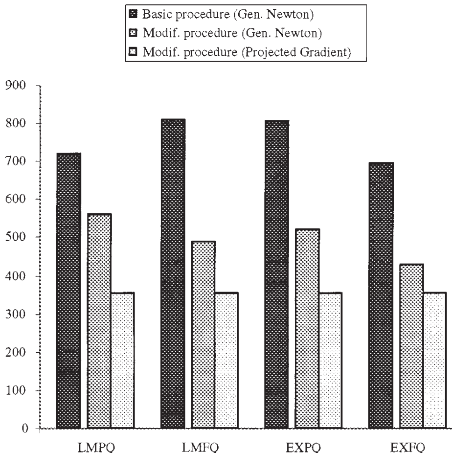
Figure 8. Number of iterations.
