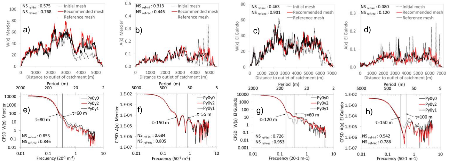
Figure 2: (a) Width-Function, W(x) , and (b) Area-Function, A(x) , of three meshes of Mercier. (ca) Width-Function, W(x) , and (d) Area-Function, A(x) , of three meshes of El Guindo. In both drainage networks came from initial mesh (segmented gray line), recommended mesh (red) and reference (black). (e) CPSD of Width-Function and (f) CPSD of Area-Function of Mercier. (g) CPSD of Width-Function and (h) CPSD of Area-Function of El Guindo. In both cases, comparing reference vs reference (PyOy0, black line), reference vs initial (PyOy1, gray segmented line) and reference vs recommended (PyOy2, red line). At six figures, NS coefficients are indicated.
