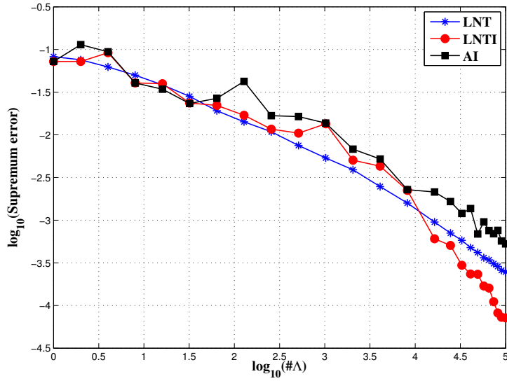
Figure 5.6: Estimated L^\infty(\mathcal{P}, V) error of LNT, LNTI and AI for the model problem (1.7) with coefficients (5.9) and d = 15 .
