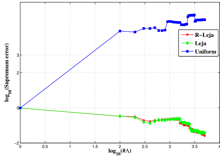
Figure 5.4: Estimated L^\infty error of the AI algorithm applied to a noisy evaluation of u_2 with d = 16 based on the sequences R , L and U .
