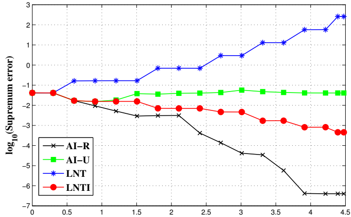
Figure 5.8: Estimated L^\infty(\mathcal{P}, V) error of LNT, of AI using U and R sequences, and of LNTI for the model problem (1.7) with coefficients (5.15) and \gamma = 0.5 .
