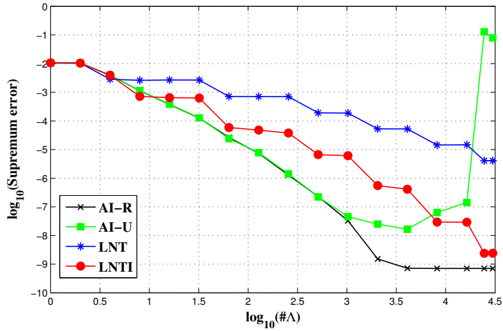
Figure 5.8: Estimated L^\infty(\mathcal{P}, V) error of LNT, of AI using U and R sequences, and of LNTI for the model problem (1.7) with coefficients (5.15) and \gamma = 0.5 .
