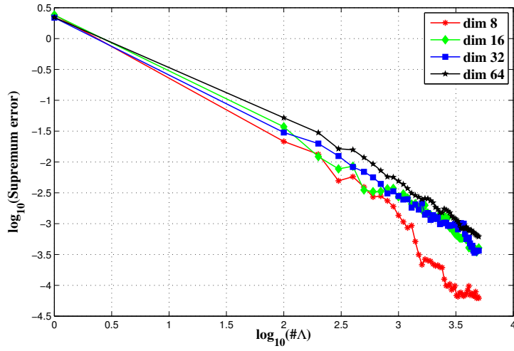
Figure 5.2: Estimated L^\infty error for the AI algorithm applied to u_2 based on the sequences R for the dimensions d = 8, 16, 32, 64 .
