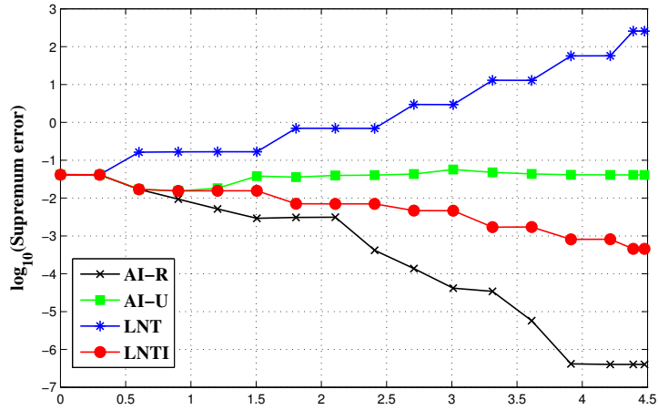
Figure 5.8: Estimated L^\infty(\mathcal{P}, V) error of LNT, of AI using U and R sequences, and of LNTI for the model problem (1.7) with coefficients (5.15) and \gamma = 0.5 .
