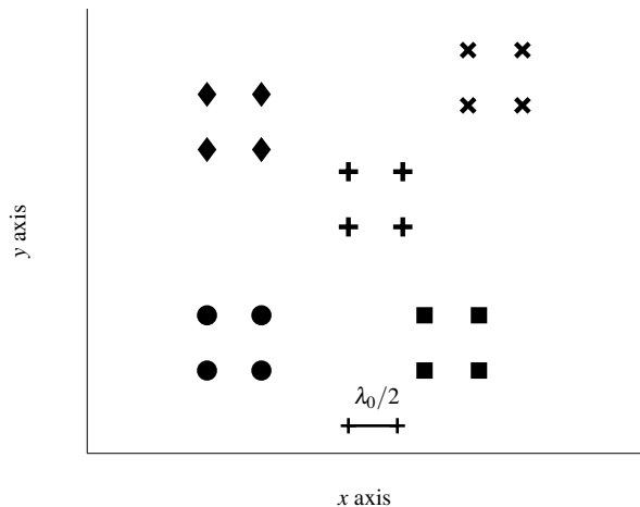
Fig. 1. Sensor position matrix - space shift diversity
