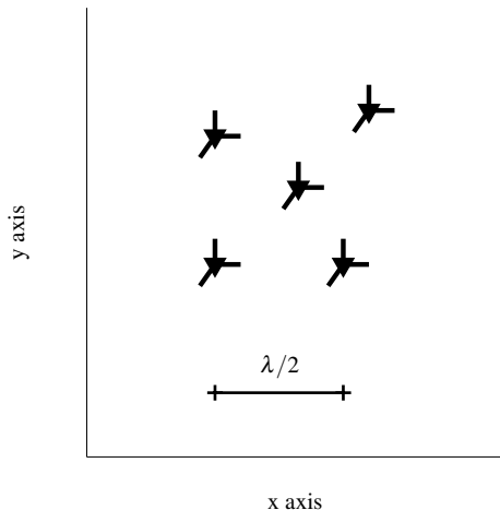
Fig. 4. 3C sensor position matrix (polarization diversity)
