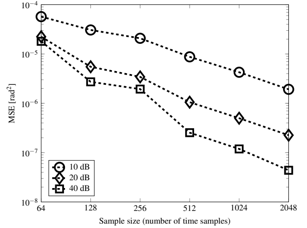
Fig. 2. MSE vs T - Narrowband tensor ESPRIT
