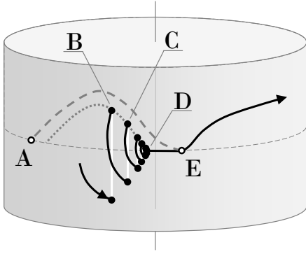
Figure 16: Sketch of a chattering trajectory (black solid curve) of the impact oscillator (6). After the first collision with the cylinder this trajectory lands on its stable manifold (dotted curve) and keeps hitting the cylinder until it accumulates at \dot{x} = 0 . The trajectory gets released after it approaches the discontinuity arc (dashed bold curve), where t \mapsto f(t, c, 0, \mu) changes sign from negative to positive.
