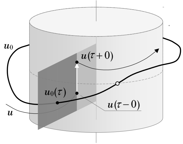
Figure 13: Periodic trajectory u_0 (bold curve) of system (6) in cylindrical coordinates, i.e. a point \zeta is assigned to u_0(t) in such a way that u_0(t) is the distance from \zeta to the vertical axis of the cylinder, \dot{u}_0(t) is the vertical coordinate of \zeta and t is the angle measured from a fixed hyperplane containing the axis of the cylinder. The surface of the cylinder is given by u = c , so that the trajectory u_0 grazes the cylinder at the point "o". The curve u is a part of the trajectory that originates from \zeta .
