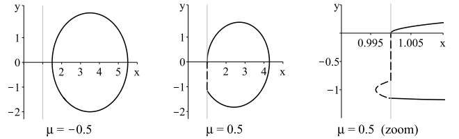
Figure 18: Stable periodic trajectories of (10) at different values of \mu . Here c = 1 , k = 0.5 , A = 1 , B = 4 .
