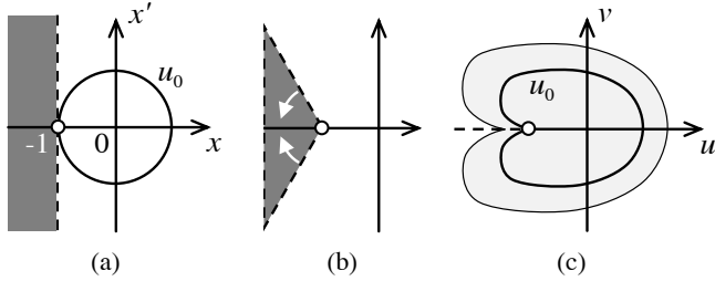
Figure 22: Statement of the problem about the topological degree of the Poincaré map \mathcal{P} over period 2\pi of (12). (a) Consider the cycle u_0 of the unperturbed system (12) that grazes the obstacle c = -1 . (b) Introduce the change of variables and bend the phase space to finally identify the positive and negative parts of the obstacle x = c . (c) The Poincaré map \mathcal{P} is now continuous in the gray region, which is a small neighbourhood of the cycle u_0 transformed according to the change of variables introduced. The problem is about evaluating the topological degree of \mathcal{P} with respect to this gray region.
