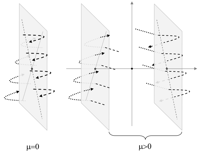
Figure 10: A partial sketch of trajectories of a 3-dimensional switching system (right graph). The limit of this sketch when the distance between the switching thresholds approach 0 (left graph).
