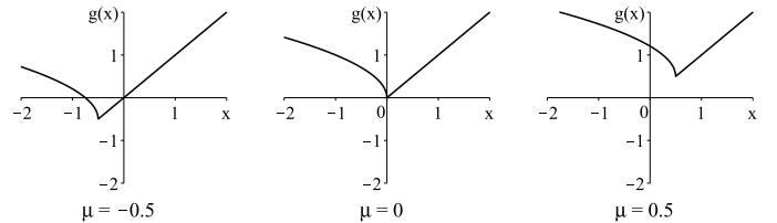
Figure 15: The map (8) at different values of the parameter \mu .
