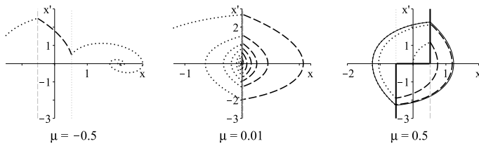
Figure 9: Trajectories of system (5) versus different values of the parameter \mu . The constant k takes the values -d and d when the trajectory crosses the dotted and the dashed lines correspondingly. These two lines can be viewed as analogues of the black and white contacts in the mechanical setup of Fig. 8. The trajectories escape from the local neighbourhood of (0,0) and converge to one of the two stable equilibria, if \mu < 0 (left graph), converge to a limit cycle, if \mu > 0 (right graph). The middle graph illustrates that the radius of the limit cycle approaches 0 when \mu \rightarrow 0 . The right graph also features the Barbashin's discontinuity surface, which is drawn in bold.
