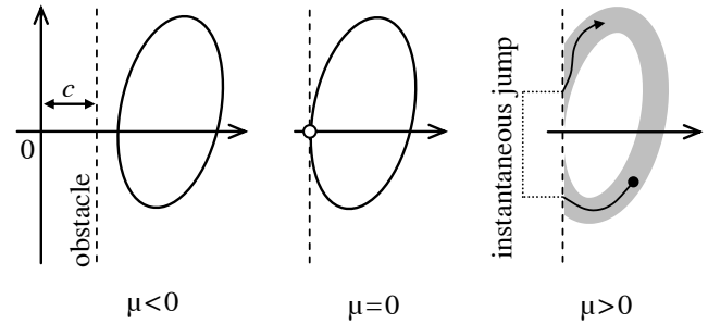
Figure 14: A stable periodic solution that exists for \mu < 0 collides with the obstacle when \mu = 0 . A grazing bifurcation occurs at this point, leading to the appearance of a trapping region (drew in gray) for small \mu > 0 . This trapping region may contain stable periodic orbits.
