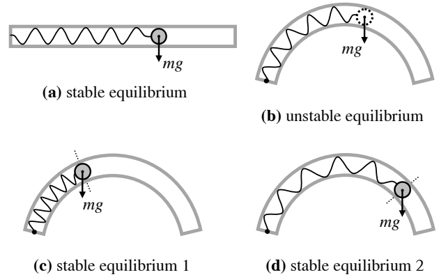
Figure 1: A ball attached to one end of a pipe subject to gravitation (directed downwards) and viscous friction.
