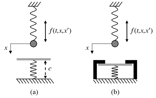
Figure 17: (a) An oscillator with one-sided spring, (b) an oscillator with one-sided preloaded spring
