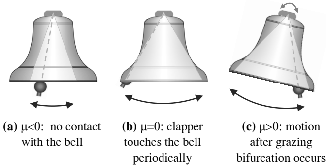
Figure 11: 3 different types of relative oscillations of the bell upon the clapper: clapper doesn't touch the bell; clapper touches the bell; clapper hits the bell
