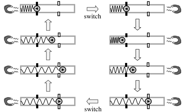
Figure 8: Illustration of a simple switching system. The right magnet activates and left magnet deactivates when the ball passes the the black contact. The opposite happens when the ball passes the white contact.
