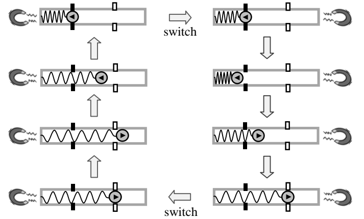
Figure 8: Illustration of a simple switching system. The right magnet activates and left magnet deactivates when the ball passes the black contact. The opposite happens when the ball passes the white contact.
