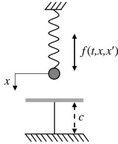
Figure 12: Impact oscillator, i.e. a ball attached to an immovable beam via a spring that oscillates upon an obstacle and subject to a vertical force f(t, u, \dot{u}) .
