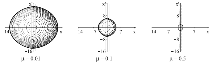
Figure 20: Stable periodic solutions of system (5) versus different values of the parameter \mu , i.e. the stable limit cycle of (5) bifurcates from infinity as the damping coefficient k deviates from 0 in the positive direction.
