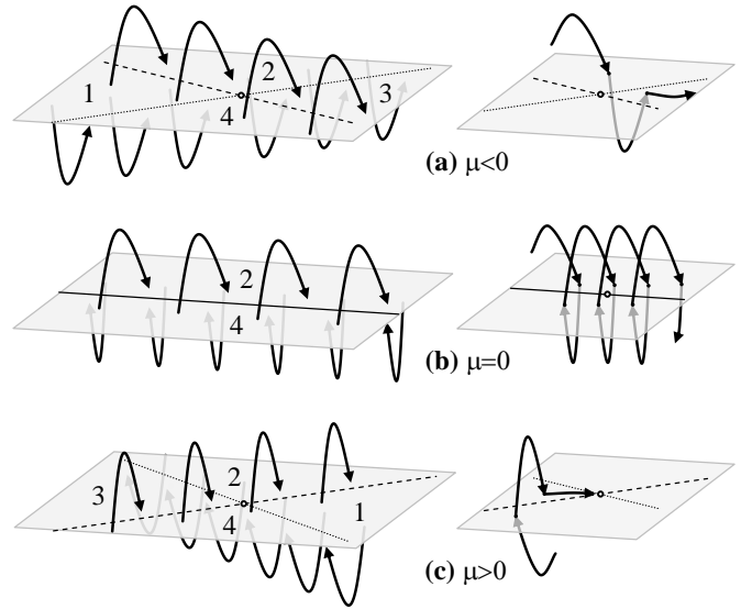
Figure 7: Teixeira singularity and its possible transformation when \mu changes through a structurally unstable situation \mu = 0 . The gray surface here is the switching hyperplane and the curves on the two sides of this hyperplane are the trajectories of two different vector fields, both of which is however tangent to the hyperplane at the point “•”.
