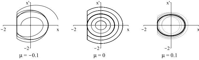
Figure 21: Trajectories of system (11) versus different values of the parameter \mu . The leftmost figure depicts an orbit that escapes from any bounded region. The middle figure shows the closed orbits of the unperturbed system (12) and the rightmost figure suggests the existence of a stable periodic solution to (11) for small positive \mu . Here k = 1 , A = 1 , r = 0 , c = -1 .
