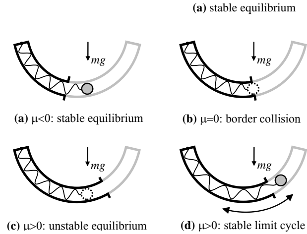
Figure 3: The pipe-ball system where the friction characteristic of the boundary changes discontinuously. The two parts where the friction characteristics is smooth are coloured in black and grey respectively. The distance between the friction discontinuity and the equilibrium of the ball is denoted by \mu . The two figures in the bottom illustrate the co-existence of an unstable equilibrium and a stable limit cycle.
