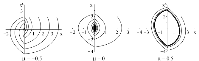
Figure 6: Trajectories of system (4) versus different values of the parameter \mu . All the trajectories converge to an interval of x = 0 , to the point (0,0) or to a cycle according to where \mu < 0 , \mu = 0 or \mu > 0 .
