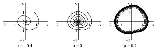
Figure 4: Trajectories of equations (1) at various values of the parameter \mu . The gray line indicates the discontinuity in the vector field (this line is located to the left or to the right from x = 0 according to whether \mu < 0 or \mu > 0 ). The trajectories converge to a point if \mu \leq 0 and to a cycle if \mu > 0 .
