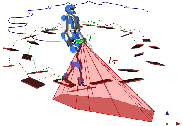
Fig. 1. HRP-4 walking on a circular staircase with tilted stepping stones using a preview controller based on 3D COM accelerations. By bounding future COM positions into a polytope \mathcal{T} (in green), we derive a trajectory-wide contact-stability condition, the COM acceleration cone I_{\mathcal{T}} (in red), that is efficiently computed with a 2D convex hull algorithm. (This cone living in acceleration space, its scale and location in the Figure above were chosen arbitrarily.) See the accompanying video [1] for demonstrations of the controller in various multi-contact scenarios.
