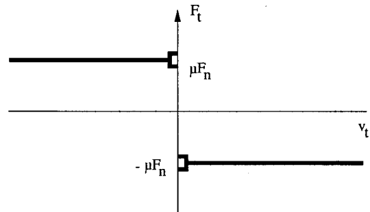
(b) The sign function
