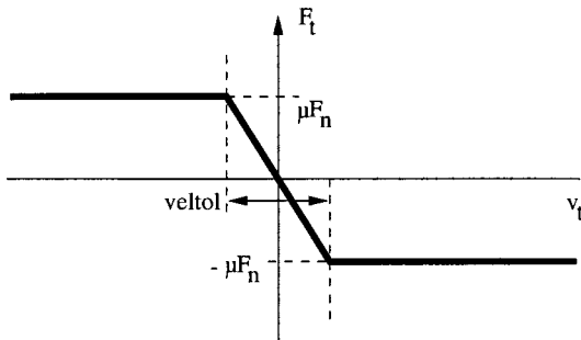
(a) A regularized Coulomb law.
