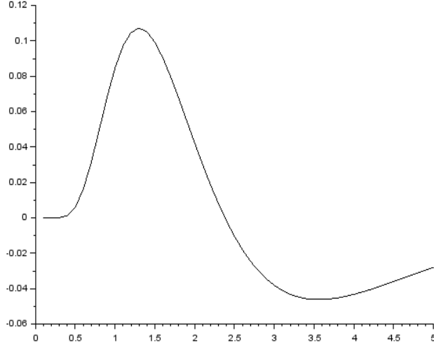
Figure 5: Graph of \alpha \mapsto h_\alpha(1) - \rho_{1,\alpha} on [0.1, 5]
