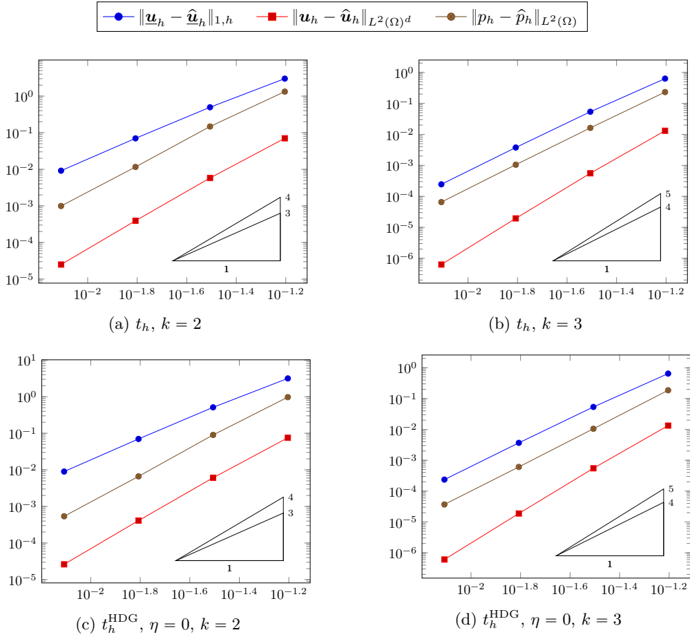
Figure 1: Cartesian mesh family, errors versus h . The triangles indicate reference slopes. The trilinear forms t_h and t_h^{\text{HDG}} are defined by (31) and (37), respectively.
