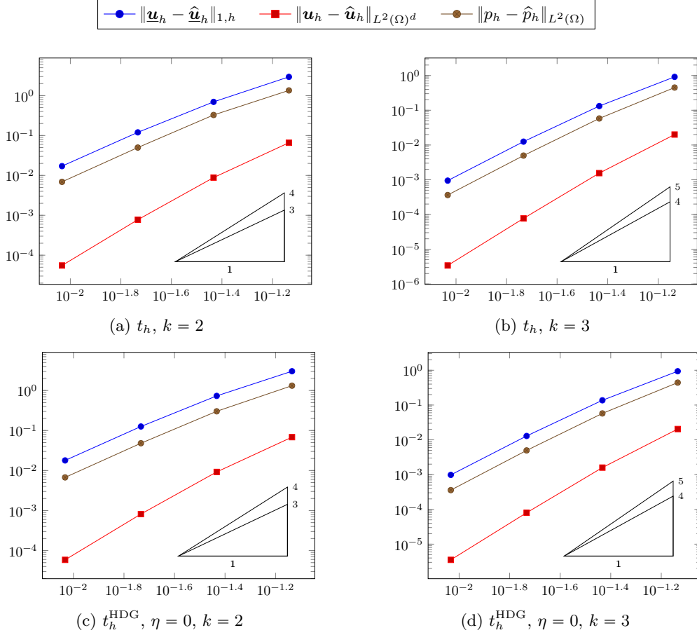
Figure 2: Hexagonal mesh family, errors versus h . The triangles indicate reference slopes. The trilinear forms t_h and t_h^{\text{HDG}} are defined by (31) and (37), respectively.
