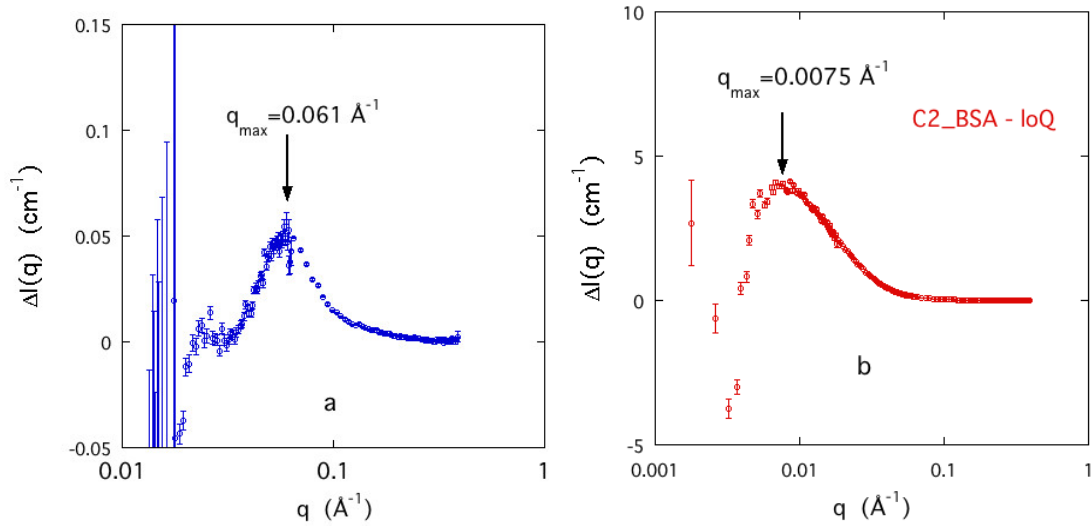
Figure S2. SANS response of the carbon samples (a) C1 and (b) C2 containing BSA at pH 6.9 from Figs. 4 and 5, after subtracting the low q response.
