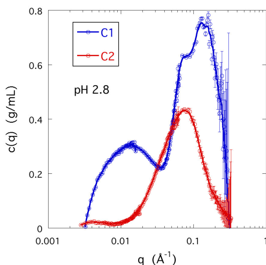
Figure S3. Distribution of protein concentration in samples C1 and C2 at pH 2.8.
