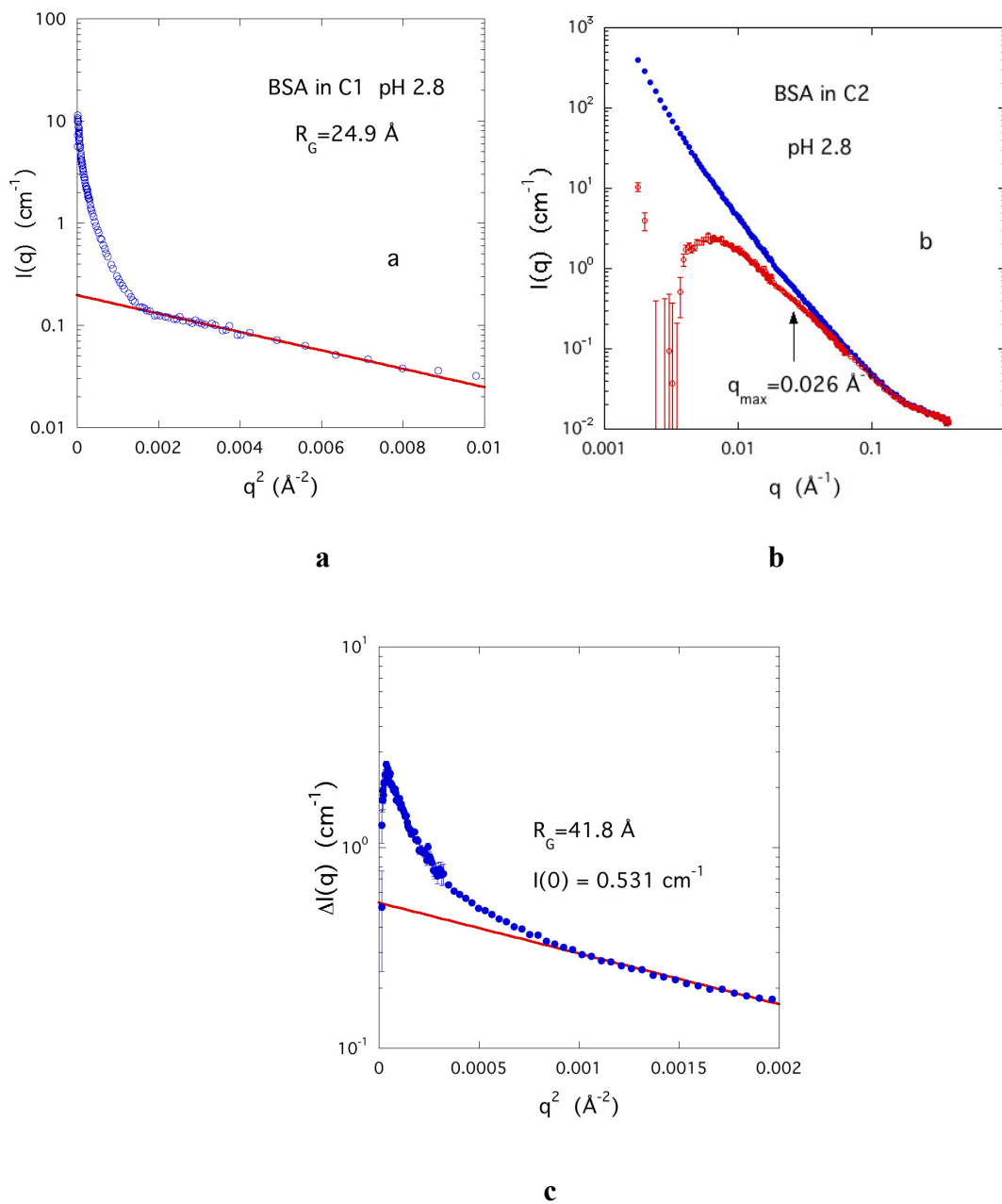
Figure 7. a) Guinier plot of the scattering intensity I(q) of BSA at pH 2.8 in the carbon aerogel C1; the extrapolated intensity of the linear behaviour is I(0) = 0.197 \text{ cm}^{-1} . b) Total intensity I(q) of BSA at pH 2.8 in carbon C2; lower curve: same data after subtraction of low- q asymptotic power law. c) Guinier plot of the data of BSA at pH 2.8 in carbon C2 in the region of the inflection at q_{\text{max}} = 0.026 \text{ \AA}^{-1} in the
