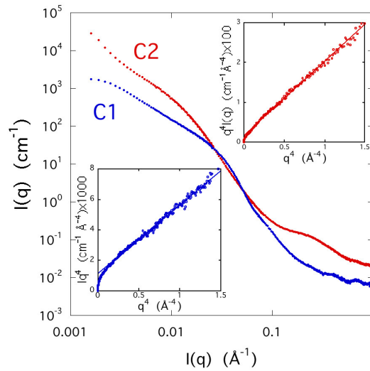
Figure S 1. SANS response of dry samples C1 and C2. Insets: plots of I(q)q^4 vs q^4 showing the intercept \kappa of the asymptotic linear region at q^4=0 . Owing to the low SANS intensity at high q in sample C1, the data shown in the corresponding inset is that measured by SAXS in an identical sample.
