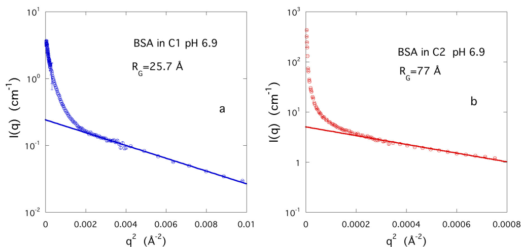
Figure 6. Guinier plots of the scattering intensity I(q) at pH 6.9 (after subtraction of the D_2O signal) in the q -region above q_{max} : (a) BSA in the carbon aerogel C1; (b) in the MAST carbon C2. The extrapolated intensities of these curves are I(0)=0.24 \text{ cm}^{-1} for BSA in C1, and I(0)=5.0 \text{ cm}^{-1} for BSA in C2.
