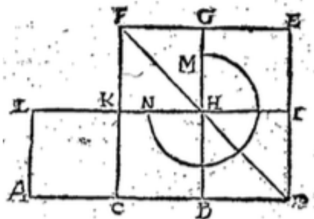
Figure 5. Geometrical interpretations of Proposition 6
