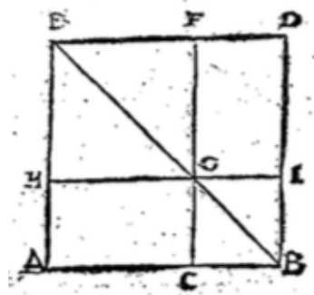
Figure 1. Geometric interpretation of Proposition 4
