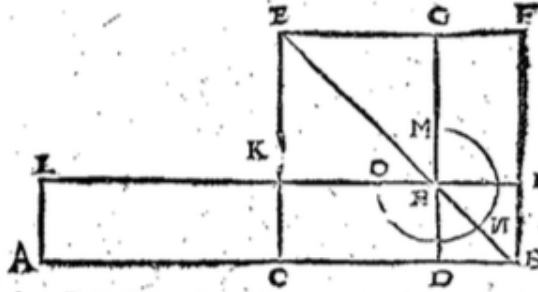
Figure 3. Geometric interpretation of Proposition 5
