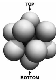
Figure 10. Kissing spheres
