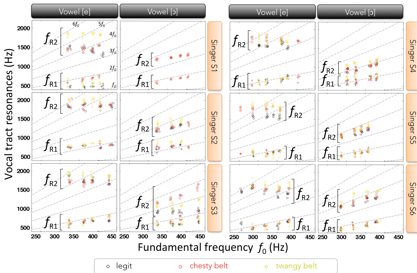
FIG. 2. (Color online) Variations of the first two vocal tract resonance frequencies ( f_{R1} and f_{R2} ) as a function of increasing pitch ( f_0 ), vowel ([e] or [ɔ]), and singing quality (legit, chesty belt, or twangy belt), for six music theatre singers. The dashed lines represent the frequency of the nearest voice harmonics ( f_0 to 6f_0 ).
