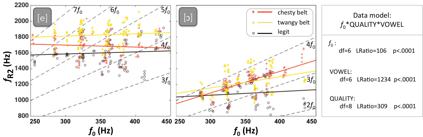
FIG. 3. (Color online) Variations of the second resonance frequency ( f_{R2} ) as a function of increasing pitch ( f_0 ), vowel ([e] or [ɔ]), and singing quality (legit, chesty belt, and twangy belt). The plain lines represent, for each quality and each vowel, the slope and intercept coefficients obtained from the regression model. The dashed lines represent the frequency of the nearest voice harmonics ( 2f_0 to 7f_0 ).
