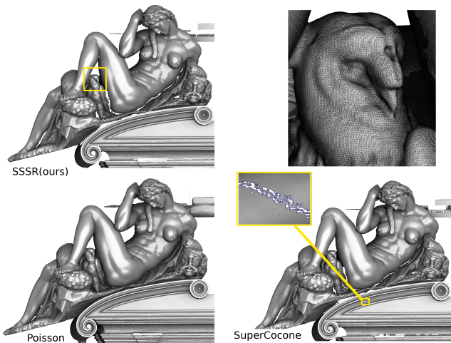
Figure 18: A dataset with 11 million vertices, extracted from a reconstruction (courtesy of the Digital Michelangelo project). Since it is not raw scanned data, the only difficulty is the number of points. Poisson creates a nice isosurface, that both respects the details and fills-in the holes (time: 230 seconds). SuperCocone gives a good result. It misses some triangles, probably in junctions between octree cells (time: 1806 seconds). Our algorithm gives a result that is similar to the output of SuperCocone in 110 seconds. ScaleSpace crashed on this dataset.
