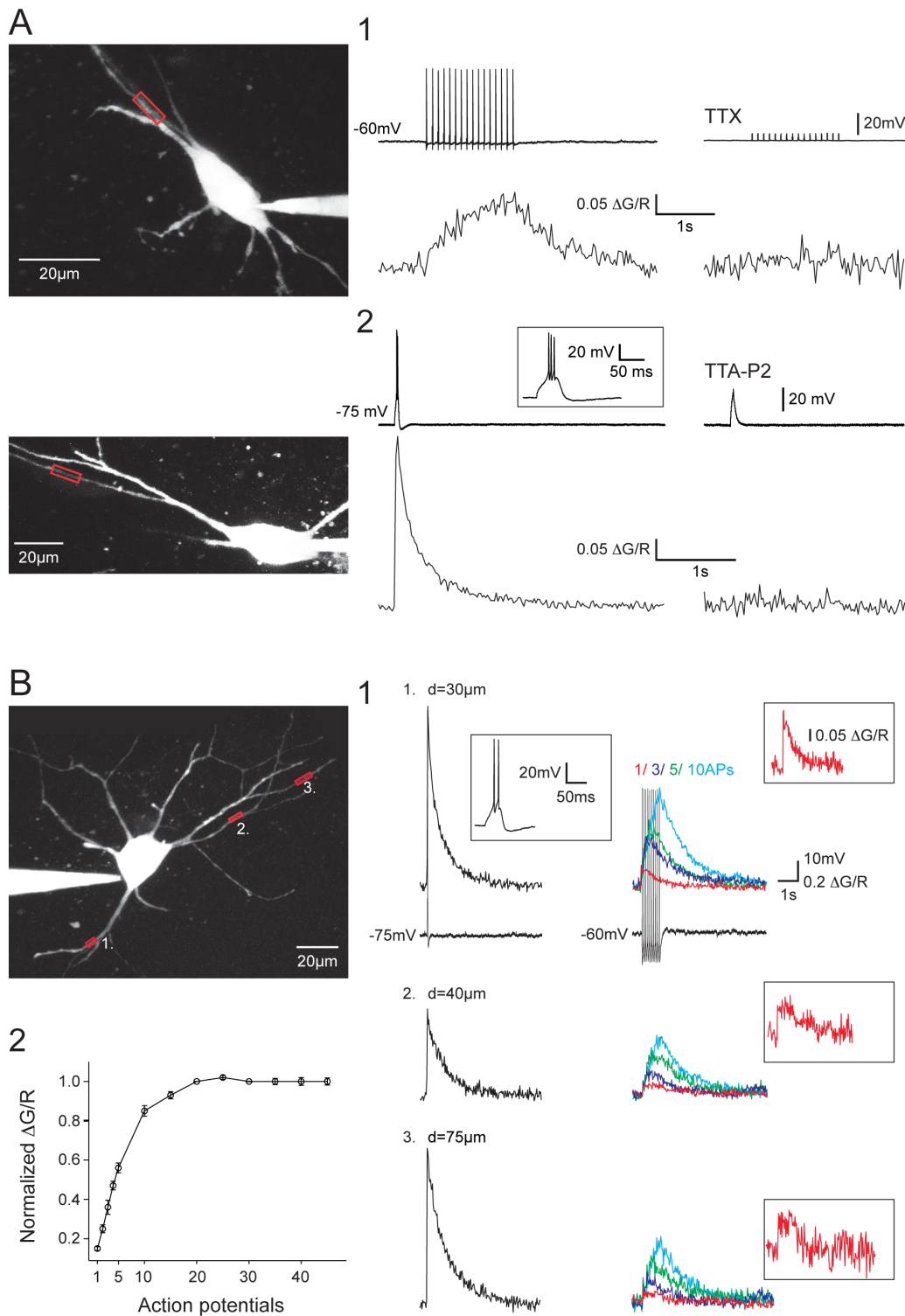
Figure 1. Dendritic Ca 2+ responses evoked by tonic APs or LTS in NRT neurons. A1. Dendritic ΔCa 2+ triggered by somatically evoked train of 15 APs at 10 Hz (top record). Application of 0.5 μM TTX fully blocked the APs and the ΔCa 2+ (bottom trace). A2. Dendritic ΔCa 2+ triggered by a somatically evoked LTS. An enlarged record of the LTS is presented in inset. Application of 3 μM TTA-P2 fully blocked the LTS and the ΔCa 2+ . B. ΔCa 2+ recorded in three different dendrites of the same neuron. B1. Dendritic ΔCa 2+ evoked by LTS (left column) and 1, 3, 5 and 10 APs at 10 Hz (right column) in the different dendrites. Examples of the somatically recorded voltage responses are shown underneath the ΔCa 2+ recorded in location 1 (an enlarged record of the LTS response is illustrated in inset). ΔCa 2+ recorded in response to a single back-propagating AP is presented at higher magnification in inset. B2. Plot of amplitude of ΔCa 2+ evoked by back-propagating APs (n = 10 neurons). The amplitude was normalized to the ΔCa 2+ evoked at the time of the 20 th AP of the trains. Note the almost linear summation of the ΔCa 2+ evoked by the first 5 back-propagating APs. In A and B the scanned dendritic regions are indicated by boxes on the maximal intensity Z projection of the neurons presented in the left panels. doi:10.1371/journal.pone.0072275.g001
