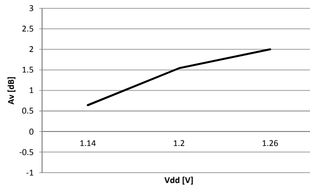
Fig. 6. Low-frequency (DC) gain vs. supply voltage.
