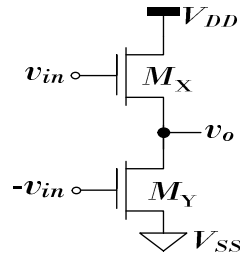
Fig. 1. VCOM circuit conceptual idea.
