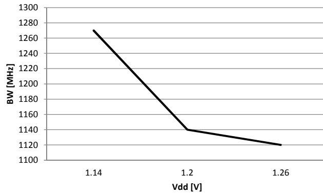
Fig. 7. Cutoff bandwidth vs. supply voltage.
