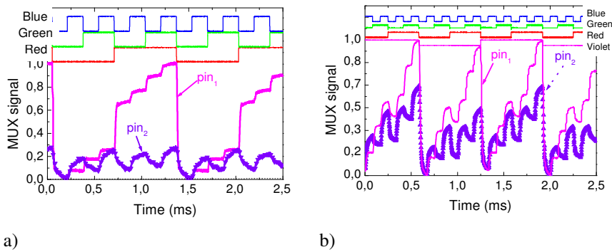
Fig. 5. Filtered output signals under front ( \text{pin}_1 ; lines) and back ( \text{pin}_2 ; symbols) violet irradiation. a) Red, Green and Blue channels. b) Red, Green, Blue and violet channels. On the top of the figures the optical signals used to transmit the information guide the eyes.
