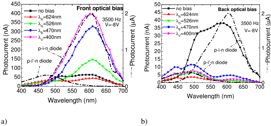
Fig. 3. Spectral photocurrent under red, green, blue and violet background irradiations (color symbols) and without it (black symbols) applied from the front (a) and back (b) diodes.
