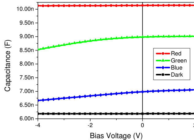
Fig. 2. - Capacitance-voltage characteristics of a pin-pin photodiode, under dark condition and under illumination with different wavelengths (red, green, and blue).
