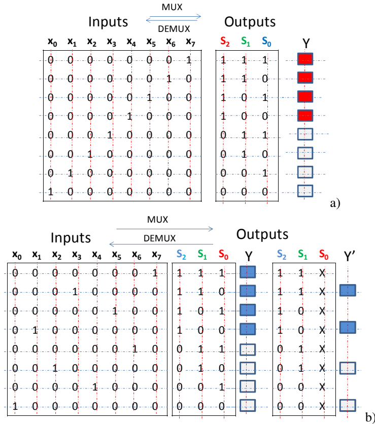
Fig. 6. Truth tables of the encoders that perform 8-to-1 multiplexer (MUX) function, under (a) front and (b) back violet irradiations (x means "not significant").
