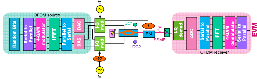
Fig.1. System Architecture of a 60 GHz OFDM-RoF with DD-MZM
