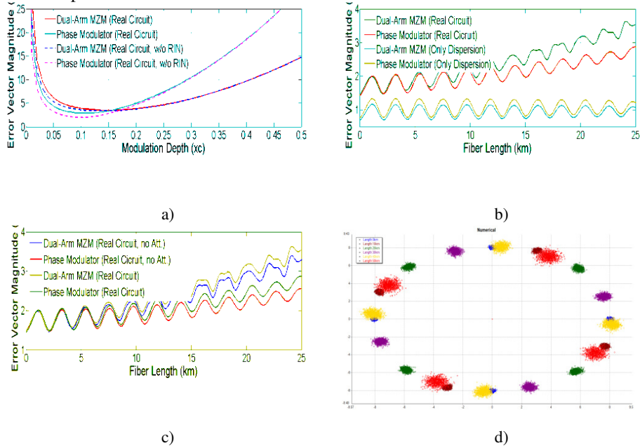
Fig.5. EVM for DD-MZM and DD-MZM cascaded with PM versus a) modulation depth for 25km of fiber length b) fiber length real conditions versus only dispersion c) fiber length real conditions versus without attenuation d) QAM constellation diagram.
