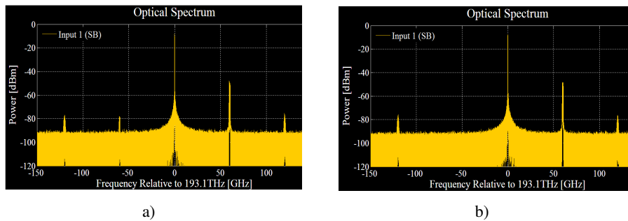
Fig.4. Optical power spectrum at a) Dual-Arm MZM ( R_{ext}=30\text{dB} ) b) Dual-Arm with PM ( R_{ext}=30\text{dB} )
