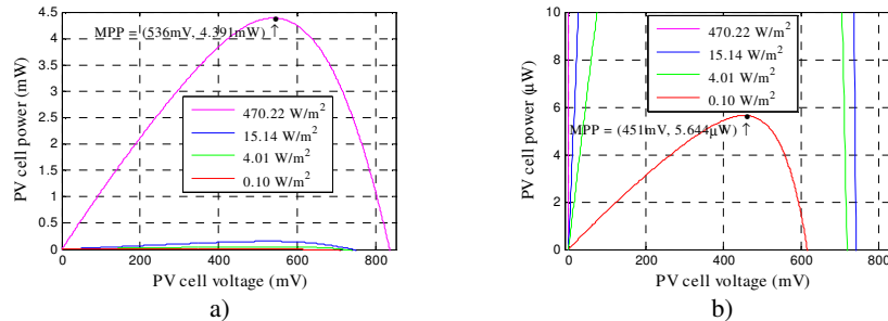
Fig.2. a) Available power from the PV cell with 1 cm 2 , for different irradiance levels. b) Detail showing the power function that corresponds to the lowest irradiance level.
