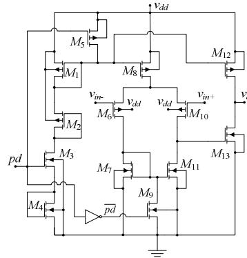
Fig.6. Differential amplifier circuit.
