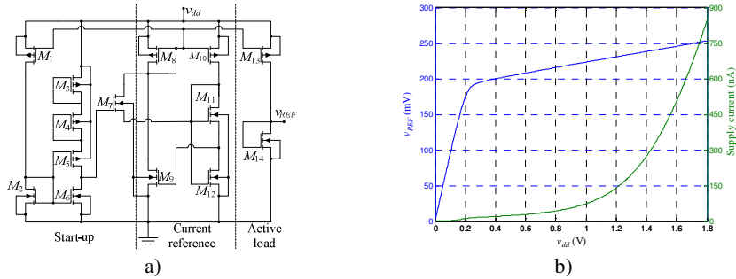
Fig.4. a) CMOS Voltage Reference Circuit. b) Output reference voltage ( v_{REF} ), and supply current, as a function of v_{dd} .
