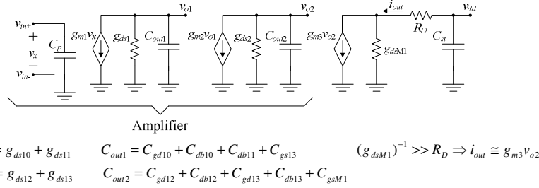
Fig.7. Small-signal model of the amplifier and the output M_1 transistor.
