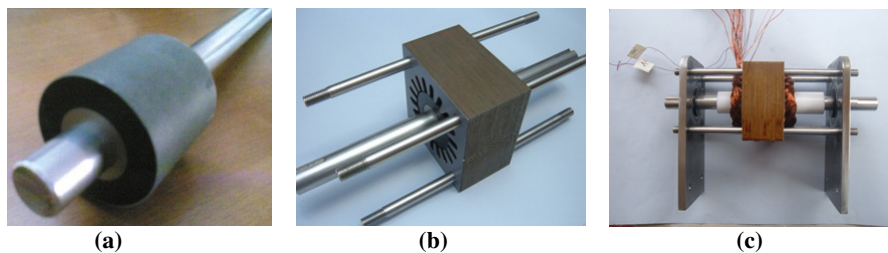
Figure 10: Constitutive parts of the assembled motor, namely (a) HTS rotor from ATZ GmbH Company with stainless steel shaft inserted; (b) stator built by stacked laminations of non-oriented silicon iron; and (c) view of the motor with terminals of 18 independent coils.
