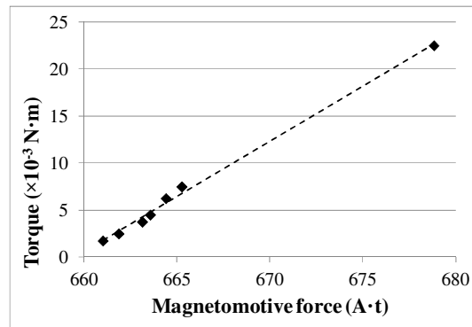
Figure 11: Comparison of developed static torques for topologies T_1 and T_2 . Torque is linear with MMF.
