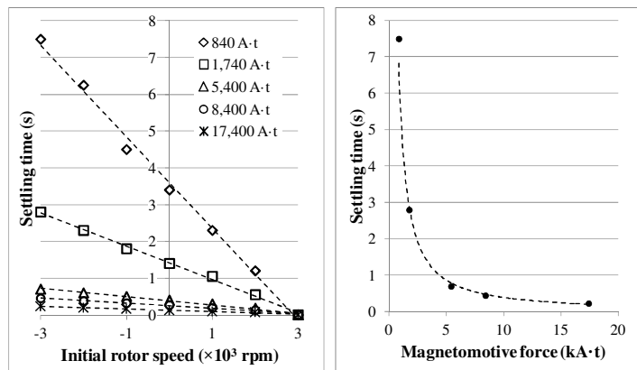
Figure 7: Settling times for topology T_1 (bipolar), as a function of (left) MMF and initial speed and (right) as a function of MMF for -3,000 rpm initial speed. Synchronous speed is 3,000 rpm. Considerably
