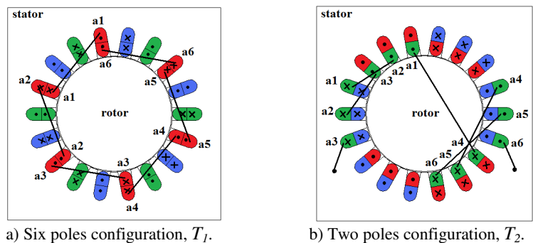
Figure 5: Different configurations in a stator with 18 slots and 18 independent coils, allowing maximum degrees of freedom in connections between windings. The stator is supplied by a three-phase system.
