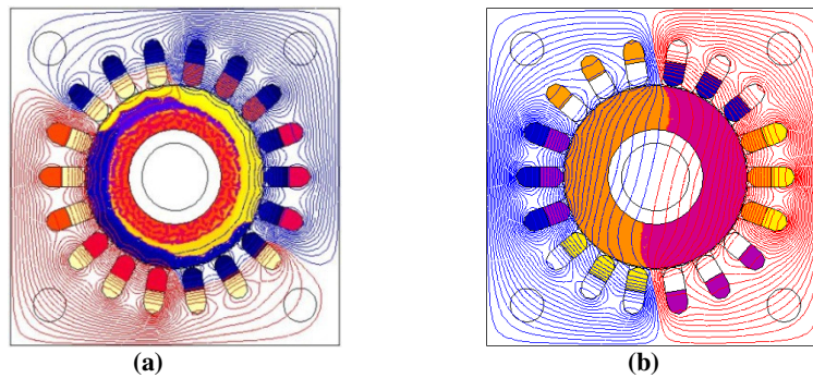
Figure 6: Profiles of current density in the rotor, for different values of MMF amplitude, corresponding to (a) partial penetration (170 A.t) and (b) full penetration (840 A.t). Superconducting properties were not a concern in simulations, only qualitative results.
