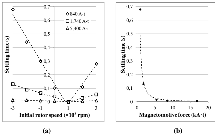
Figure 8: Settling times for topology T_2 (hexapolar), as a function of (a) MMF and initial speed, where results above 5,400 A-t are not shown as they overlap, and (b) as a function of MMF for -3,000 rpm initial speed. Synchronous speed is 1,000 rpm.
