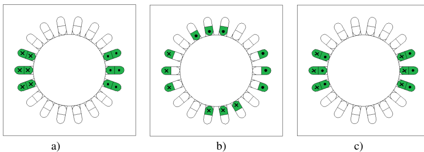
Figure 4: Geometrical displacement of two windings of the same phase, in a double layer stator.
