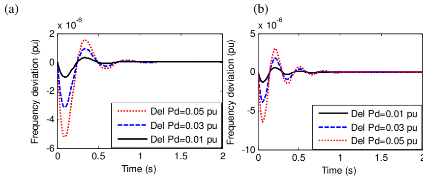
Fig. 3. Frequency deviation for ALQR (a) and CLQR (b) with load disturbances.
