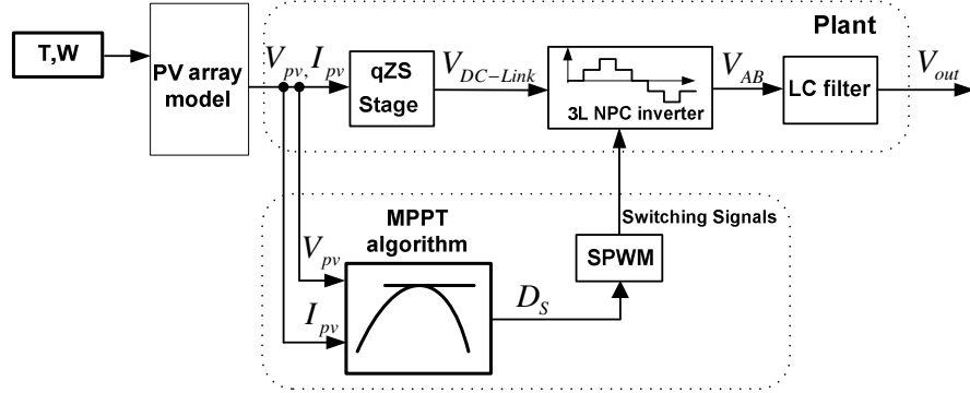
Fig. 1. General block-diagram of the analyzed photovoltaic system.
