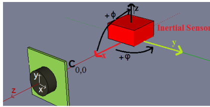
Fig. 3. Inertial and camera C_{0,0} referential
