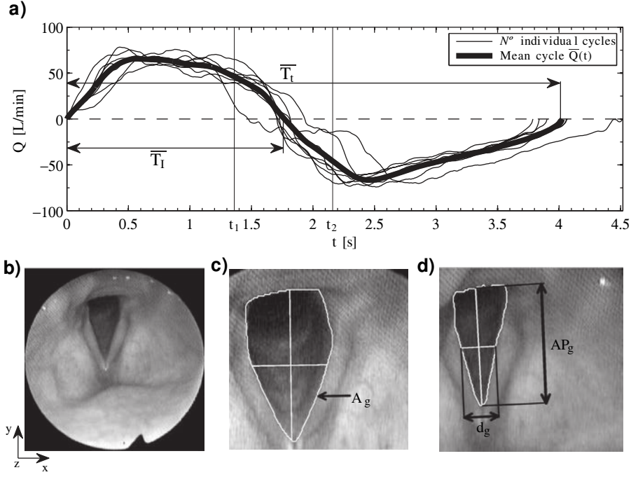
Fig. 1. (a) Superposed individual breathing cycles Q(t) (subject M01, task Eup 15 ) and resulting mean breathing cycle in function of time t [s]. (b) Example of laryngoscopic area. Corresponding contour of glottal area A_g , antero-posterior diameter AP_g and glottal width d_g at the time of maximum opening t_1 (c) and at time of minimum opening t_2 (d).
