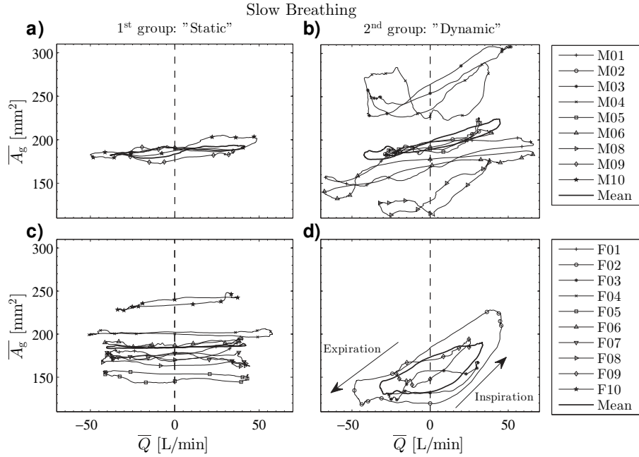
Fig. 4. Glottal area variations during slow breathing . Upper panels (a and b) are for male subjects, and lower panels (c and d) are for female subjects. Left panels (a and c) are dedicated to the 1st group (with “static” glottal movement) and right panels (b and d) are dedicated to the 2nd group (with “dynamic” glottal movement).
