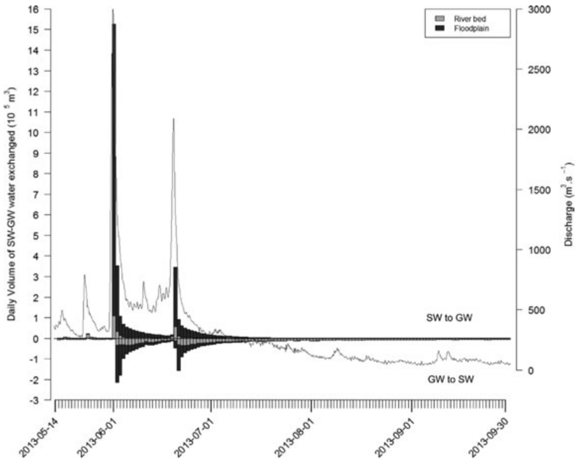
Fig. 8. Daily exchanged water volume between SW and GW (positive values for infiltration, negative values for exfiltration). Dark grey represents exchanges for the plain area, and light grey for the riverbed area. Hourly discharge is shown by a black solid line.
