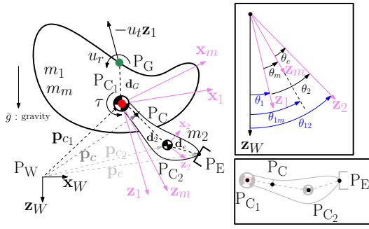
Fig. 1: Left: a sketch of the PVTOL equipped with an actuated link. Notice the offset between the CoM of the PVTOL ( P_{C_1} , red point) and the center of actuation ( P_G , green point). The rigid link is attached to P_{C_1} , around which the motor rotates and a either rigid or elastic joint is placed, i.e. P_{C_1} = P_M . Right-up: relative and absolute angles of the rigid bodies, where the length of the \mathbf{z} axes are made different just for better illustration. Right-down: locations of important points on the arm.
