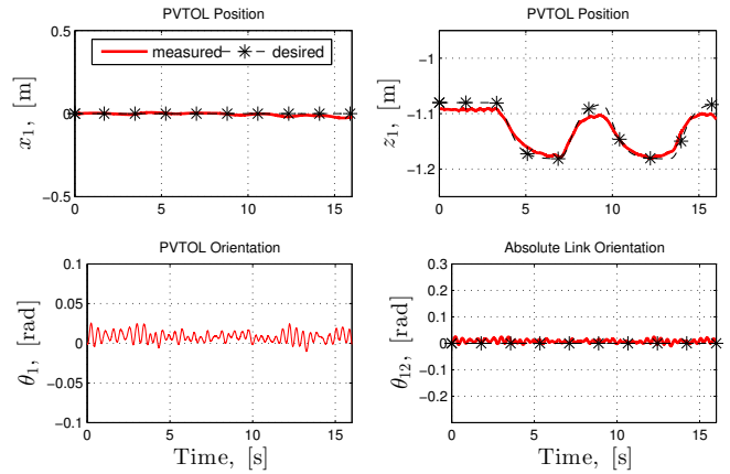
Fig. 4: First test on controlling the Quadrotor + VSA arm position along x and z directions. A step-like trajectory is followed along the z -axis. Notice that negative z is upwards.
