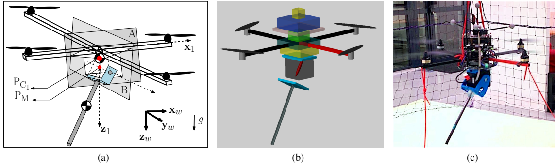
Fig. 3: Evolution from theory to application. a) Conceptual sketch of the model in 3D. The motion in Plane-A is controlled using the controller presented in this paper. The motion in Plane-B (except the translational motion along z_1 ) and the rotation around z_1 is controlled using a near-hovering controller [26]. b) CAD model of the 3D system and a snapshot from SimMechanics simulation, where the implemented controllers have been tested. Different colors correspond to the different parts of the real system. The results are given in the video attachment of this paper. c) Real system on flight. On board of the VTOL, from top to bottom, there are MoCap markers, an Odroid-XU computer, four brushless motor controllers with their power board, a flight controller (incl. IMU), battery pack, Qbmove with its connectors, a rigid arm attached to it. Red ropes are used only for safety reasons, with no tension on them.
