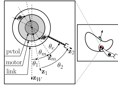
Fig. 2: An ideal example of elastic joint between the motor output shaft and link. Proportions are distorted for illustration purposes. The innermost circle, fixed to \mathcal{F}_1 , represents the PVTOL. The middle circle, fixed to \mathcal{F}_M , represents the actuator (or motor). The outermost circle is connected to the middle circle via elastic components, and it is rigidly connected to the link (fixed to \mathcal{F}_2 .)
