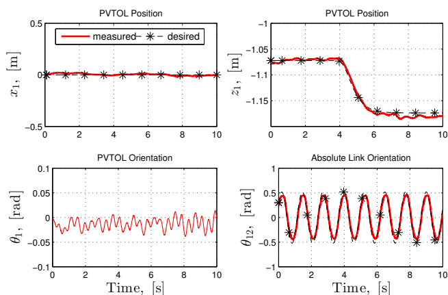
Fig. 5: Preliminary results for trajectory tracking with Quadrotor+VSA arm setup. The arm attached to the Qbmove is swinging back and forth (see \theta_{12} ), while Quadrotor VTOL is tracking a stable trajectory along x -direction, and a step-like trajectory along the z -direction. Oscillations on \theta_1 are due to the motion of the arm, against which controller is trying to keep x position constant. Notice that negative z is upward.
