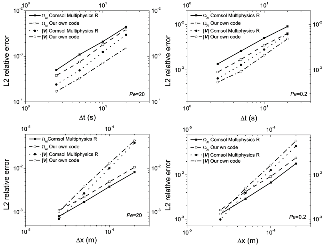
Fig. 9. Temporal and spatial L^2 -norm relative errors of the solutions using Comsol Multiphysics ® and our own code under Pe = 20 and Pe = 0.2 .
