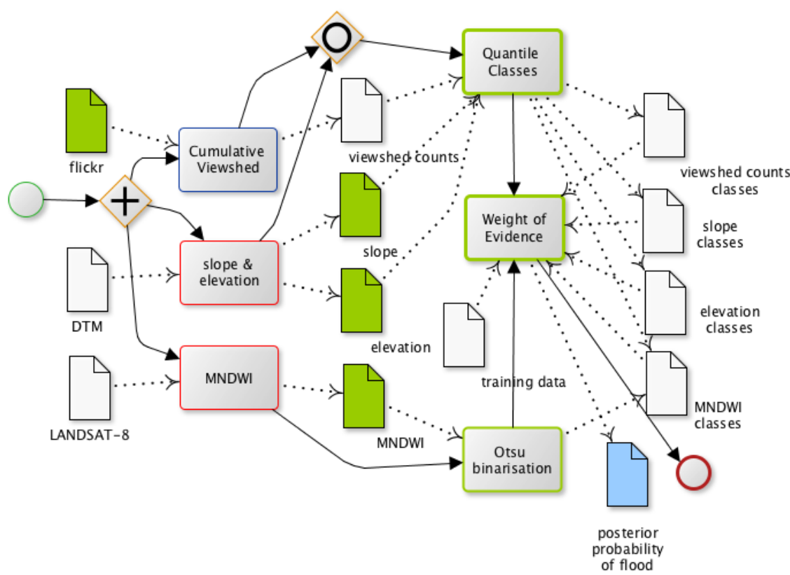
Figure 1: BPMN workflow of the rapid flood inundation data fusion method used in Rosser et al. (2016) – in green are the data input where uncertainty sampling takes place.
