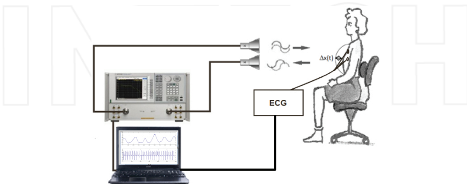
Figure 1. Proposed system design: microwave system and ECG.
