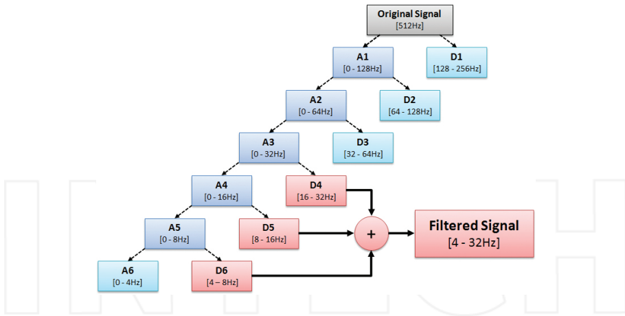
Figure 4. Example of wavelet decomposition.
