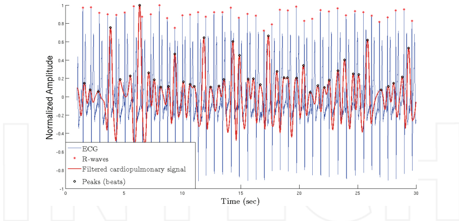
Figure 5. ECG vs. cardiopulmonary signal extracted from the front side of the subject and processed using DWT Bior2.4 level 8.
