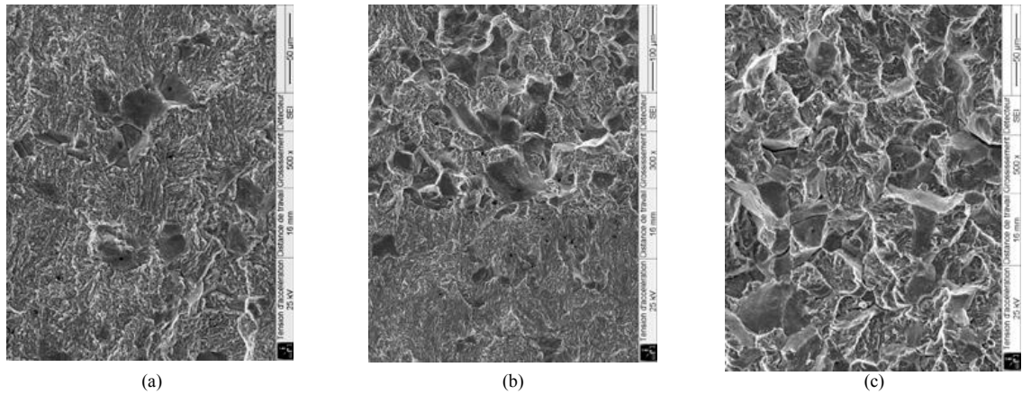
Fig. 5. Crack surface morphology under 4 bars hydrogen atmosphere; (a) in the near threshold domain; (b) \Delta K = 14 \text{ MPa}\sqrt{\text{m}} with a sharp transition in the crack propagation mechanism; (c) \Delta K = 30 \text{ MPa}\sqrt{\text{m}} . (Propagation from bottom to top).
