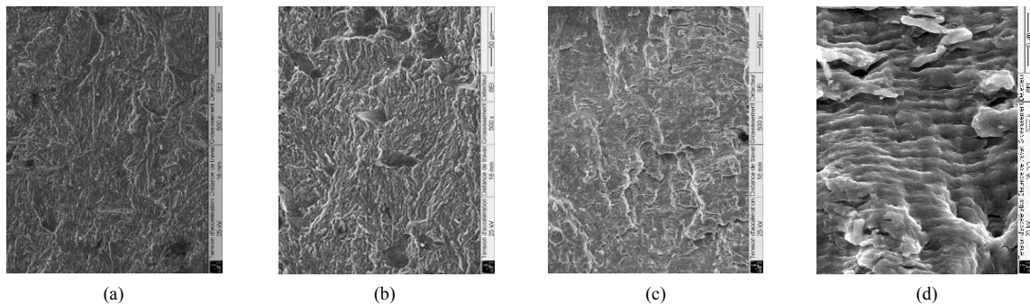
Fig. 3. Micrographic aspect of fracture surface in ambient air (a) near the threshold; (b) \Delta K = 14 \text{ MPa}\sqrt{\text{m}} ; (c) \Delta K = 50 \text{ MPa}\sqrt{\text{m}} ; (d) magnification of striations. (Propagation from bottom to top).
