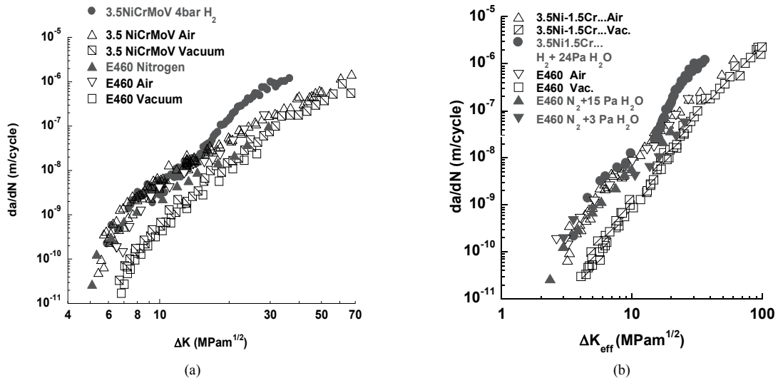
Fig.6. Comparison of the influence of environment on 3.5NiCrMoV in hydrogen with 24Pa of water vapor and E460 steel in Nitrogen with 15Pa and 3 Pa of water vapor, with reference high vacuum ( <5 \cdot 10^{-4} \text{ Pa} ) and ambient air with \sim 150 \text{ Pa} of water vapor; (a) nominal curves; (b) effective curves.
