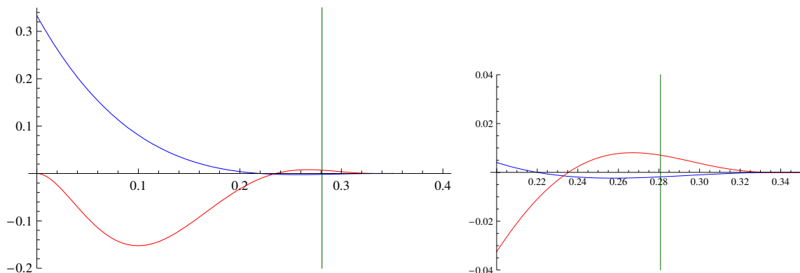
Figure 5. The functions \Delta_1(\gamma, r = r_+(\gamma)) (blue) and \Delta_2(\gamma, r = r_+(\gamma)) (red) rescaled by a \equiv \frac{3\lambda_2|c|C}{h^2} and a^2 , respectively. ( \Delta_2 was also multiplied by 10 to make it more visible.) The vertical line indicates the bound \gamma < \gamma_* in (4.16). The right picture magnifies the region near the critical value. Both pictures demonstrate that, in the allowed range of \gamma , the two functions are never simultaneously positive.
