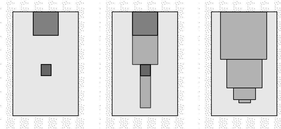
FIGURE 3. The doubling property. On the left, the cylinders Q_{\omega/4} and Q_{\omega/2}(0, 0, 1) . In the middle, the elongated cylinders Q^0 and Q^1 . On the right, the iterated cylinders Q^0, \dots, Q^N (Lemma 23).
