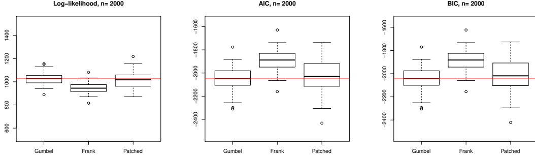
FIGURE 4. Boxplots for the log-likelihood, AIC and BIC criteria for the 3 considered models (true Gumbel model, initial Frank model and patched distorted model). In the red horizontal line we display the median values for the Gumbel model. We consider M = 100 Monte Carlo simulations.
