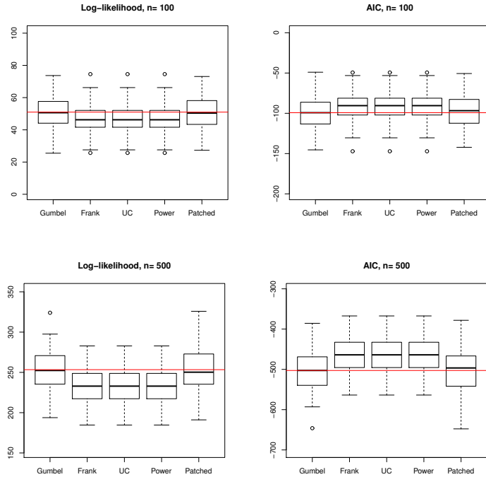
FIGURE 8. Boxplots for the log-likelihood and Akaike information criterion (AIC) for true Gumbel, initial Frank, upper-comonotonic, power distortion and patched model. Sample sizes n = 100 (first row) and n = 500 (second row). In the red horizontal line we display the median values for the Gumbel model. We consider M = 100 Monte Carlo simulations.
