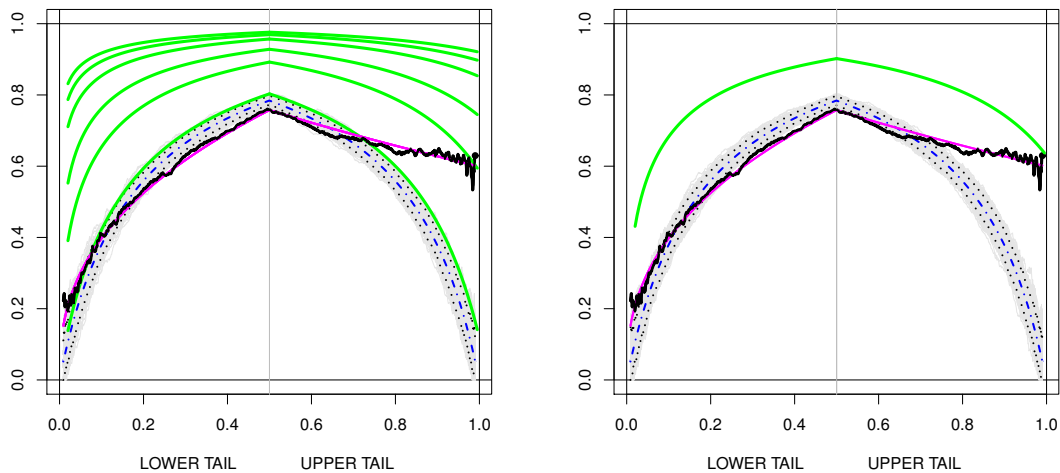
(A) with arbitrary chosen \beta 's values from the top \beta = 9, 7, 5, 3, 2 and \hat{\beta}_{ML} = 1.095 (B) with \hat{\beta} = 2.199901 such that the \lambda_{\hat{\beta}} = \hat{\lambda}_U = 0.63
