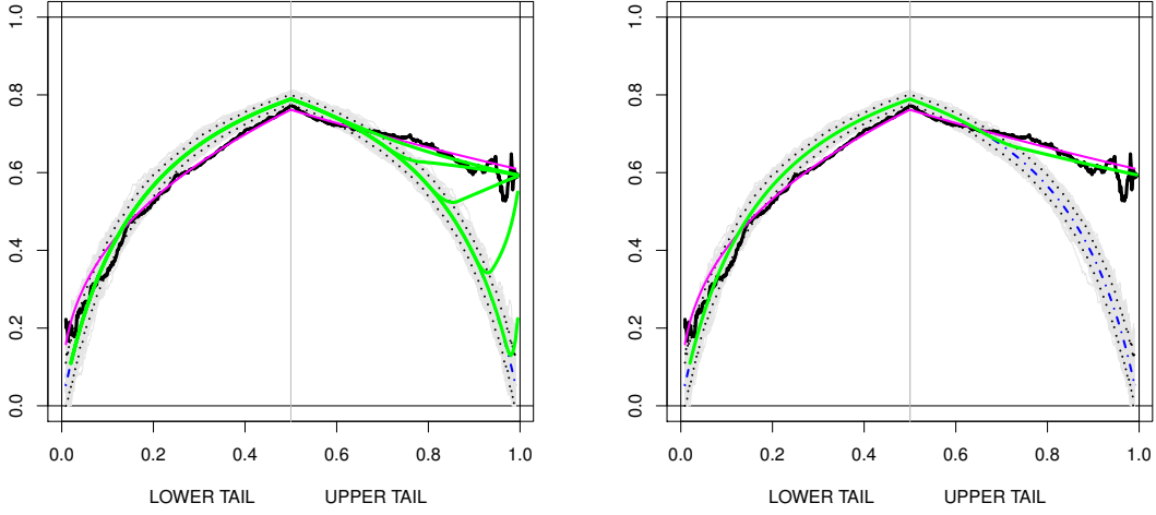
(A) with arbitrary chosen u^* 's values.
