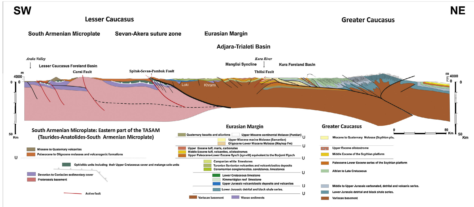
Fig. 2. Crustal section across the Greater and Lesser Caucasus (see location on Fig. 1). Active faults in Lesser Caucasus are from Avagyan et al. (2005, 2010). Ophiolites are obducted over the southern Armenian Microplate over a minimum distance of 120 km. The schistosity in the inner part of the Greater Caucasus is indicated on the section (unpublished results from our group).
