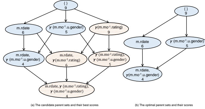
Figure 4: Score' propagation and pruning in the relational parent graph of Movie.genre .
