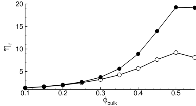
FIGURE 12. Relative viscosity \eta_r as a function of volume fraction ( \kappa=20 ) for friction coefficients \mu_d=0 ( \circ ) and \mu_d=0.5 ( \bullet ).
