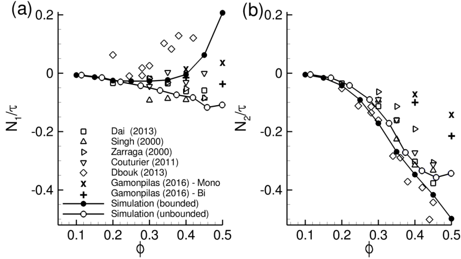
FIGURE 20. Normal stress differences N_1 (a) and N_2 (b) normalized by shear stress \tau as a function of volume fraction for a frictional suspension \mu_d=0.5 : bounded suspension \kappa=20 ( \bullet ) and unbounded suspension ( \circ ). Experiments (symbols) compile results from Zarraga et al. (2000); Singh & Nott (2000); Dbouk et al. (2013); Dai et al. (2013); Couturier et al. (2011); Gamonpilas et al. (2016). Data from Gamonpilas et al. (2016) are for monomodal particles (Mono) and bimodal mixture (Bi).
