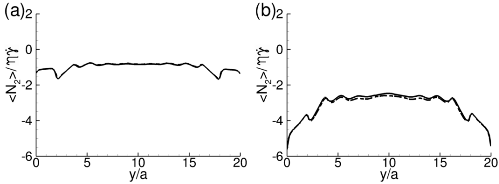
FIGURE 18. Particle-phase average \langle N_2(y) \rangle / \eta \dot{\gamma} (solid lines) and \langle N_2^c(y) \rangle / \eta \dot{\gamma} (dotted lines) in a suspension at \phi_{bulk}=0.4 and \kappa=20 for two friction coefficients : \mu_d=0 (a) ; \mu_d=0.5 (b).
