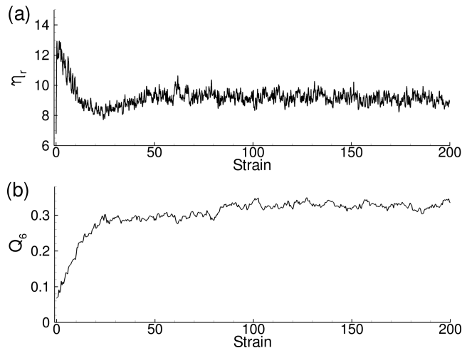
FIGURE 11. Relative viscosity \eta_r (a) and parameter Q_6 (b) as a function of strain \gamma = \dot{\gamma}_{bulk}t . Simulations at \phi_{bulk}=0.5 , \kappa=20 and \mu_d=0 .
