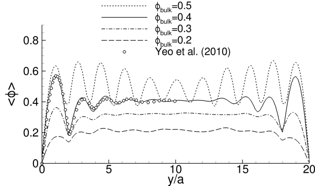
FIGURE 4. Local volume fraction \langle \phi(y) \rangle in the channel width for \kappa=20 and bulk fractions \phi_{bulk} = (0.2, 0.3, 0.4, 0.5) . Open symbols are computations by Yeo & Maxey (2010b).
