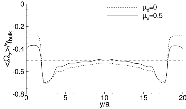
FIGURE 10. Particle-phase angular velocity \langle \Omega_z(y) \rangle / \dot{\gamma}_{bulk} for frictionless particles \mu_d=0 (dotted lines) and frictional particles \mu_d=0.5 (solid lines). Simulations at \phi_{bulk}=0.4 and \kappa=20 . Dashed line is -\dot{\gamma}_{bulk}/2 .
