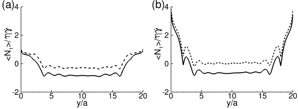
FIGURE 15. Particle-phase average \langle N_1(y) \rangle / \eta \dot{\gamma} (solid lines) and \langle N_1^c(y) \rangle / \eta \dot{\gamma} (dotted lines) in a suspension at \phi_{bulk}=0.4 and \kappa=20 for two friction coefficients : \mu_d=0 (a) ; \mu_d=0.5 (b).
