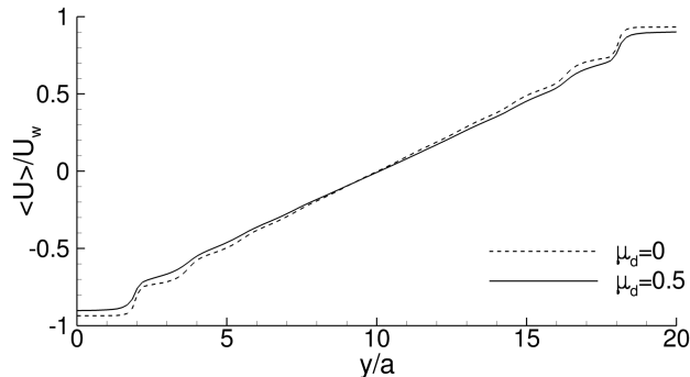
FIGURE 8. Particle-phase axial velocity \langle U(y) \rangle / U_w for frictionless particles \mu_d=0 (dotted lines) and frictional particles \mu_d=0.5 (solid lines). Simulations at \phi_{bulk}=0.4 and \kappa=20 .
