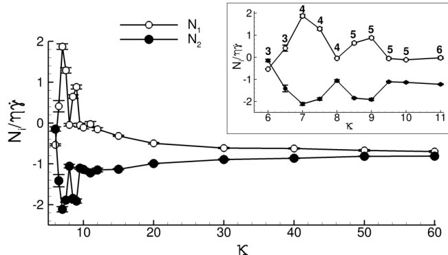
FIGURE 22. Effect of confinement \kappa on normal stress differences N_1/\eta\dot{\gamma} ( \circ ) and N_2/\eta\dot{\gamma} ( \bullet ) at \phi_{bulk}=0.4 and \mu_d=0 in the range 6 \leq \kappa \leq 60 . (Inset : range 6 \leq \kappa \leq 11 ; the bold numbers indicate the number of layers).
