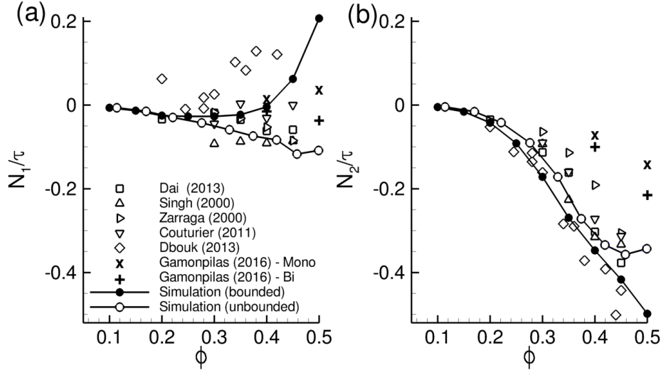
FIGURE 20. Normal stress differences N_1 (a) and N_2 (b) normalized by shear stress \tau as a function of volume fraction for a frictional suspension \mu_d=0.5 : bounded suspension \kappa=20 ( \bullet ) and unbounded suspension ( \circ ). Experiments (symbols) compile results from Zarraga et al. (2000); Singh & Nott (2000); Dbouk et al. (2013); Dai et al. (2013); Couturier et al. (2011); Gamonpilas et al. (2016). Data from Gamonpilas et al. (2016) are for monomodal particles (Mono) and bimodal mixture (Bi).
