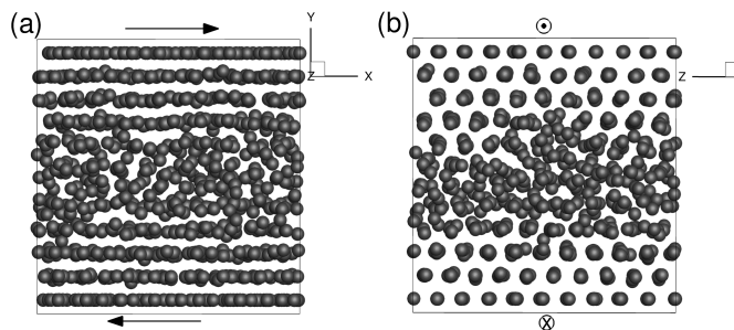
FIGURE 3. Particle snapshots ( \phi_{\text{bulk}}=0.5 ; \kappa=20 ; \mu_d=0 ): (a) side view; (b) end view. For visualization, particle radius is half the actual size.
