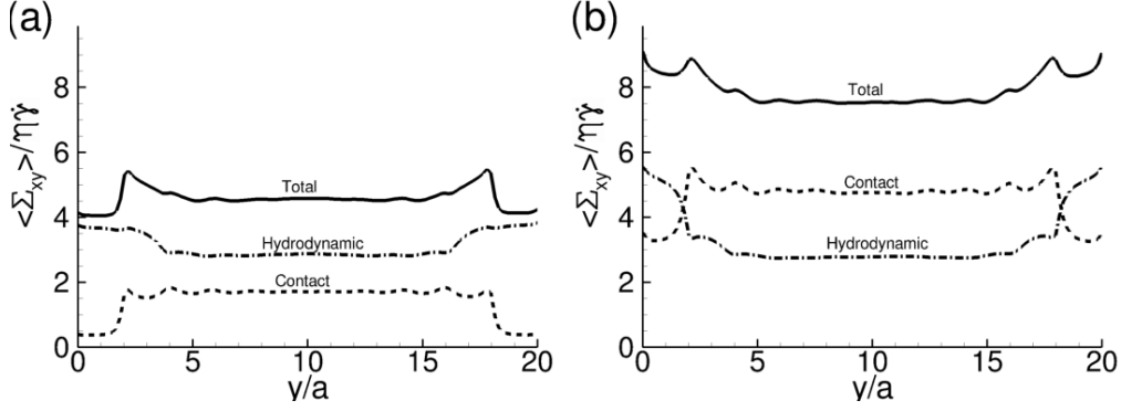
FIGURE 13. Particle-phase particle stress \langle \Sigma_{xy}^p(y) \rangle / \eta \dot{\gamma} (solid lines), hydrodynamic stress \langle \Sigma_{xy}^h(y) \rangle / \eta \dot{\gamma} (dash-dotted lines) and contact stress \langle \Sigma_{xy}^c(y) \rangle / \eta \dot{\gamma} (dotted lines) in a suspension at \phi_{bulk} = 0.4 and \kappa = 20 for two friction coefficients : \mu_d = 0 (a) ; \mu_d = 0.5 (b)
