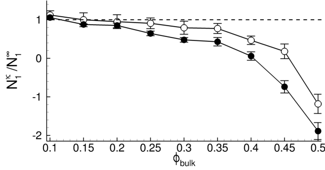
FIGURE 17. Ratio of bounded to unbounded N_1^kappa/N_1^infinity as a function of volume fraction for \mu_d=0 ( \circ ) and \mu_d=0.5 ( \bullet ) for \kappa=20 .
