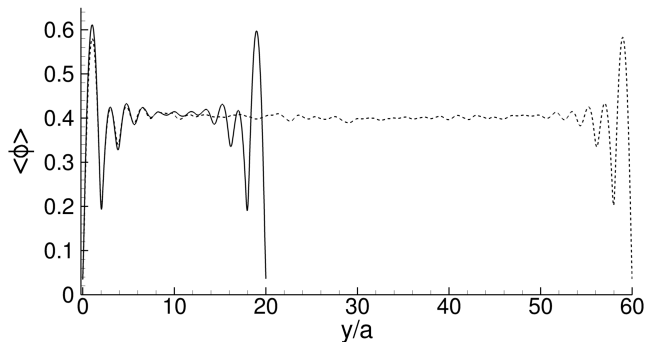
FIGURE 6. Volume fraction profile \langle\phi(y)\rangle for \kappa=20 (solid lines) and \kappa=60 (dotted lines). Simulations at \phi_{bulk}=0.4 and \mu_d=0 .
