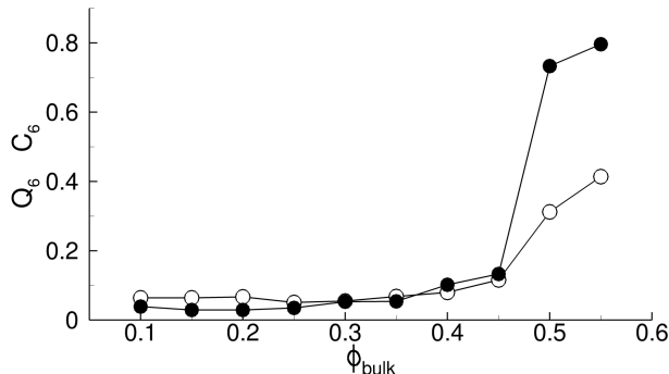
FIGURE 2. Order parameters Q_6 (○) and C_6 (●) as a function of volume fraction ( \kappa=20 ; \mu_d=0 ).
