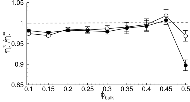
FIGURE 14. Ratio of bounded to unbounded viscosity \eta_r^\kappa / \eta_r^\infty as a function of volume fraction for \mu_d = 0 (o) and \mu_d = 0.5 (•) for \kappa = 20 .
