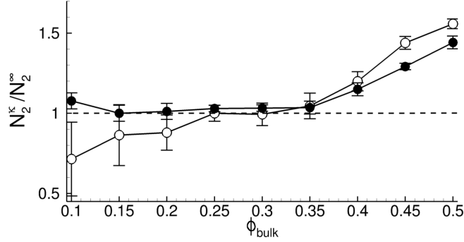
FIGURE 19. Ratio of bounded to unbounded N_2^\kappa / N_2^\infty as a function of volume fraction for \mu_d=0 ( \circ ) and \mu_d=0.5 ( \bullet ) for \kappa=20 .
