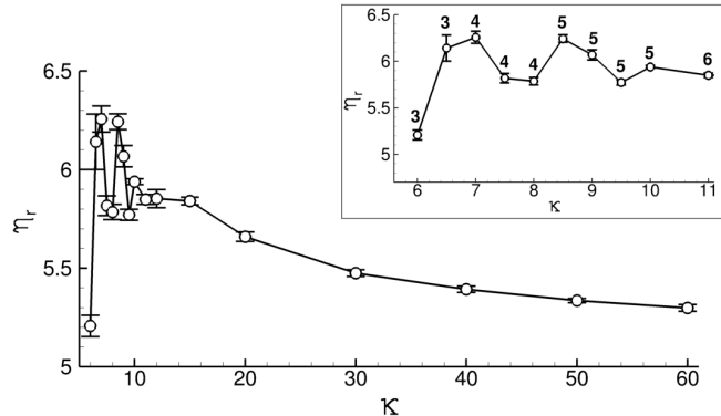
FIGURE 21. Effect of confinement \kappa on viscosity \eta_r at \phi_{bulk}=0.4 and \mu_d=0 in the range 6 \leq \kappa \leq 60 . (Inset : range 6 \leq \kappa \leq 11 ; the bold numbers indicate the number of layers).
