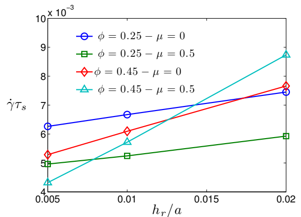
FIG. 14. Selected representative values of the reduced relaxation time \dot{\gamma}\tau_s of particle normal forces as a function of particle roughness h_r/a .
