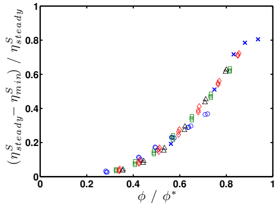
FIG. 11. Difference between steady and minimum suspension viscosity \eta_{steady}^S - \eta_{min}^S to the steady \eta_{steady}^S suspension viscosity as a function of reduced volume fraction \phi/\phi^* . Simulations with h_r/a \in [5.10^{-3}; 10^{-2}; 2.10^{-2}] and \phi \in [0.25; 0.3; 0.35; 0.4; 0.45; 0.5] : ( \circ ) \mu = 0 , ( \square ) \mu = 0.3 , ( \diamond ) \mu = 0.5 , ( \triangle ) \mu = 0.7 , ( \times ) Experiments \phi^* = 0.53 - a = 15.5 \mu m [27].
