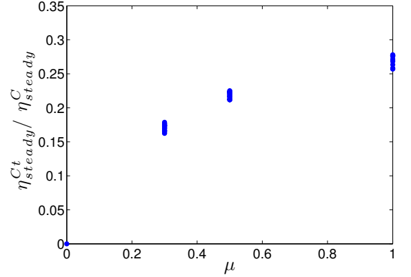
FIG. 18. Ratio of the tangential contribution \eta_{steady}^{Ct} to the total contact \eta_{steady}^C viscosity as a function of friction coefficient \mu . 0.2 \leq \phi \leq 0.5 , 5.10^{-3} \leq h_r/a \leq 2.10^{-2} .
