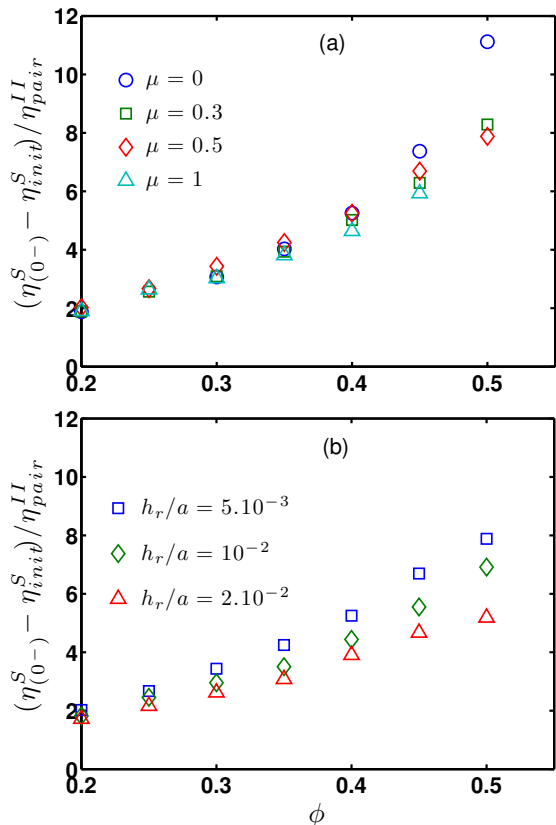
FIG. 19. Ratio of the viscosity step \eta_{(0-)}^S - \eta_{init}^S to the expected step from particle pair model \eta_{pair}^{II} (Eq. 36) as a function of solid volume fraction (a) h_r/a = 5 \cdot 10^{-3} (b) \mu = 0.5
