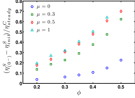
FIG. 17. Ratio of the jump in relative viscosity (\eta_{0-}^S - \eta_{init}^S) to the steady contact viscosity \eta_{steady}^C . h_r/a = 5.10^{-3} .
