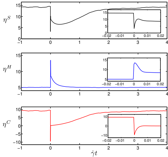
FIG. 3. The relative viscosity \eta^S of a suspension under shear reversal \phi = 0.45 , \mu = 0.5 , h_r/a = 5.10^{-3} as a function of shear strain \dot{\gamma}t (top), together with the hydrodynamic contribution \eta^H (middle) and contact contribution \eta^C (bottom) from Eq. (24). The inset shows the fast dynamics due to the relaxation of the contact forces. The shear reversal takes place at t = 0 .
