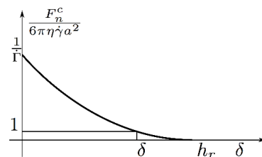
FIG. 2. Normalized contact force as a function of surface-to-surface distance \delta . \delta is the typical surface-to-surface distance.
