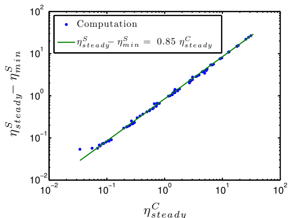
FIG. 10. Difference between steady and minimum suspension viscosity \eta_{steady}^S - \eta_{min}^S as a function of steady contact viscosity \eta_{steady}^C . 0.25 \leq \phi \leq 0.5 , h_r/a = 5.10^{-3} ; 10^{-2} ; 2.10^{-2} , \mu = 0 ; 0.3 ; 0.5 ; 1 .
