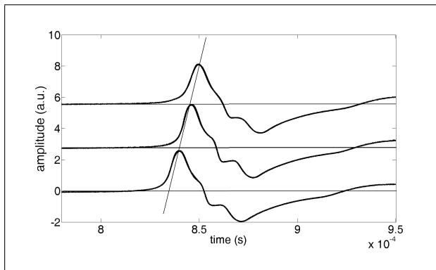
Figure 8. Example of 3 waveforms propagating along the surface of a poroelastic cylinder in the case of pulse excitation. The signals were detected at different distances from the source in steps of \Delta x = 0.028 mm. The curves are plotted with an off-set for clarity.
