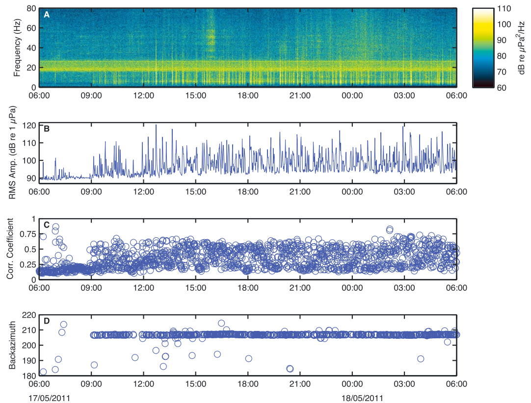
Figure 2. Twenty-four hours of data recorded at station H10S, beginning at 06:00 UTC 17 May 2011. (a) Single-receiver spectrogram of the H10S1 hydrophone data. A 2 Hz high-pass filter is applied to eliminate low-frequency noise; however, wide-band contamination is present between 18 and 26 Hz, possibly due to ship noise. (b) Root-mean-squared (RMS) amplitudes calculated over 1 min windows. The results of the time-difference-of-arrival processing are shown in the form of (c) correlation coefficients and (d) back azimuths averaged over the H10S array. Only time windows with an average coefficient \geq 0.33 are used in the back azimuth calculation. The onset of the eruption at Monowai is recognizable in all four subfigures: Hydroacoustic phases, most distinguishable in the 2 to 20 Hz band, arrive from 09:00 UTC onward, accompanied by a positive shift in RMS amplitude of almost 20 dB re 1 \mu\text{Pa} . Correlation values between hydrophones increase significantly at the same time, resulting in the distinct stabilization of the angle of arrival to within a degree of the predicted back azimuth to Monowai at 205.5^\circ .
